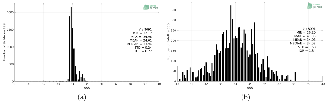
Figure 2: Histograms of SSS from Saildrone (a) and SMOS SSS L2Q v331 - 0.25 Deg (CATDS-CPDC) (b) considering all match-up pairs per bins of 0.1 over the Roaring Forties and Furious Fifties Pi-MEP region and for the full satellite product period.
