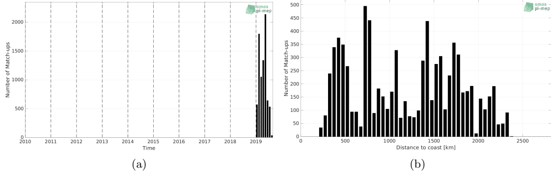
Figure 1: Number of match-ups between Saildrone and SMOS SSS L2Q v331 - 0.25 Deg (CATDS-CPDC) SSS as a function of time (a) and as function of the distance to coast (b) over the Roaring Forties and Furious Fifties Pi-MEP region and for the full satellite product period.
