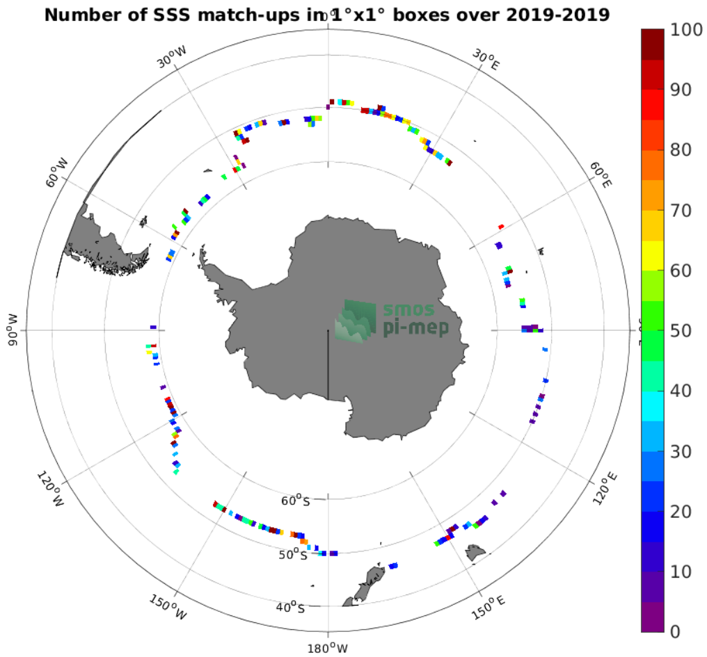
Figure 4: Number of SSS match-ups between Saildrone SSS and the SMOS SSS L2Q v331 - 0.25 Deg (CATDS-CPDC) SSS product for the Roaring Forties and Furious Fifties Pi-MEP region over 1°x1° boxes and for the full satellite product period.
