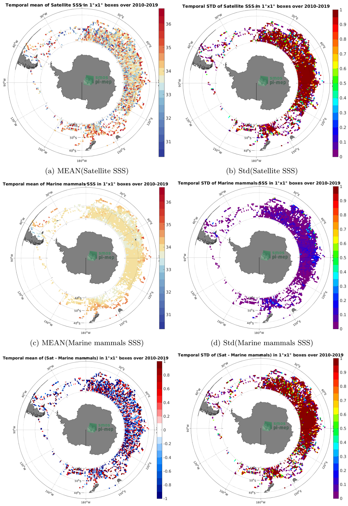
Figure 6: Temporal mean (left) and Std (right) of SSS from SMOS SSS L2Q v331 - 0.25 Deg (CATDS-CPDC) (top), Marine mammals (middle), and of \Delta SSS (Satellite - Marine mammals). Only match-up pairs are used to generate these maps.
