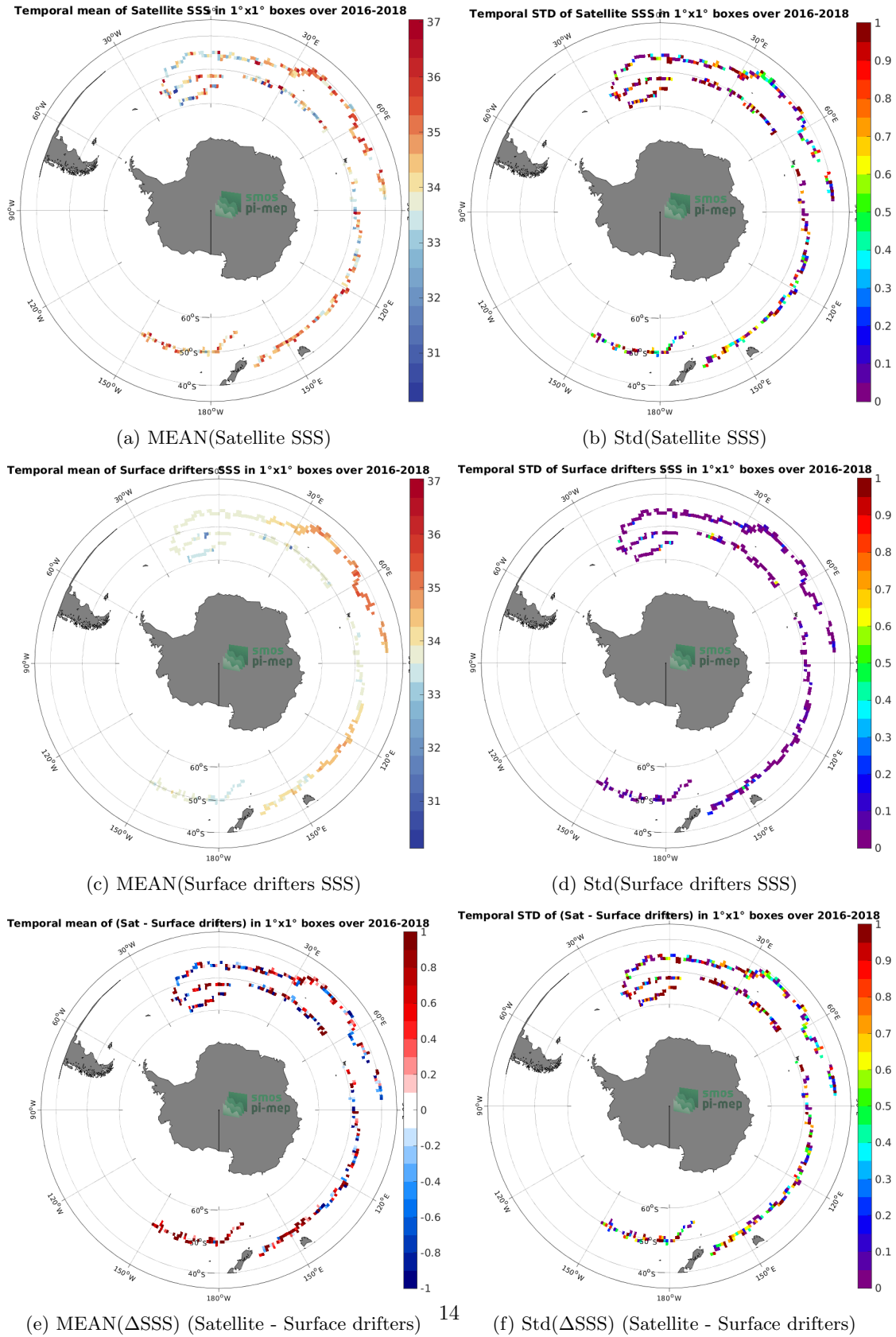
Figure 5: Temporal mean (left) and Std (right) of SSS from SMOS SSS L2Q v331 - 0.25 Deg (CATDS-CPDC) (top), Surface drifters (middle), and of \Delta SSS (Satellite - Surface drifters). Only match-up pairs are used to generate these maps.
