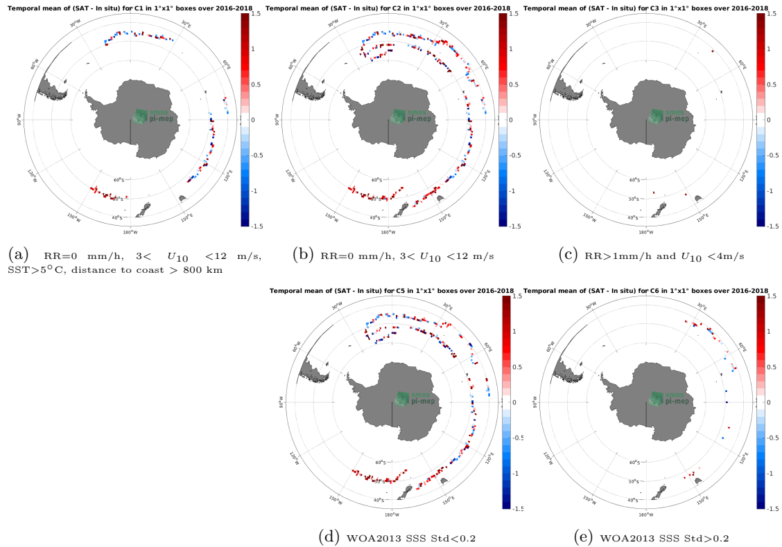
Figure 11: Temporal mean gridded over spatial boxes of size 1^{\circ}\times 1^{\circ} of \Delta\text{SSS} (SMOS SSS L2Q v331 - 0.25 Deg (CATDS-CPDC) - Surface drifters) for 5 different subdatasets corresponding to:RR=0 mm/h, 3 < U_{10} < 12 m/s, SST >5^{\circ}\text{C} , distance to coast > 800 km (a), RR=0 mm/h, 3 < U_{10} < 12 m/s (b), RR >1 mm/h and U_{10} < 4 m/s (c), WOA2013 SSS Std <0.2 (d), WOA2013 SSS Std >0.2 (e).
