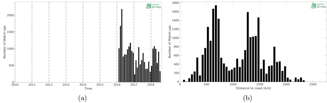
Figure 1: Number of match-ups between Surface drifters and SMOS SSS L2Q v331 - 0.25 Deg (CATDS-CPDC) SSS as a function of time (a) and as function of the distance to coast (b) over the Roaring Forties and Furious Fifties Pi-MEP region and for the full satellite product period.
