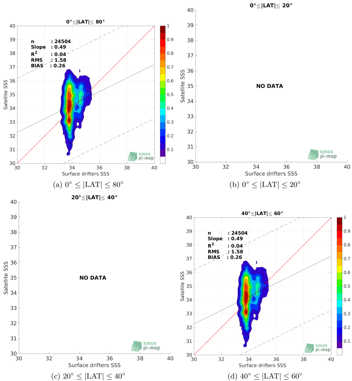
Figure 8: Contour maps of the concentration of SMOS SSS L2Q v331 - 0.25 Deg (CATDS-CPDC) SSS (y-axis) versus Surface drifters SSS (x-axis) at match-up pairs for different latitude bands. For each plot, the red line shows x=y . The black thin and dashed lines indicate a linear fit through the data cloud and the \pm 95\% confidence levels, respectively. The number match-up pairs n , the slope and R^2 coefficient of the linear fit, the root mean square (RMS) and the mean bias between satellite and in situ data are indicated for each latitude band in each plots.
