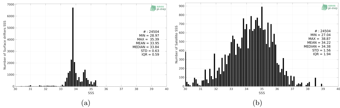
Figure 2: Histograms of SSS from Surface drifters (a) and SMOS SSS L2Q v331 - 0.25 Deg (CATDS-CPDC) (b) considering all match-up pairs per bins of 0.1 over the Roaring Forties and Furious Fifties Pi-MEP region and for the full satellite product period.
