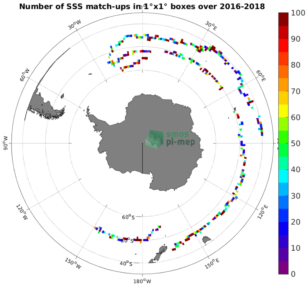
Figure 3: Number of SSS match-ups between Surface drifters SSS and the SMOS SSS L2Q v331 - 0.25 Deg (CATDS-CPDC) SSS product for the Roaring Forties and Furious Fifties Pi-MEP region over 1^\circ \times 1^\circ boxes and for the full satellite product period.
