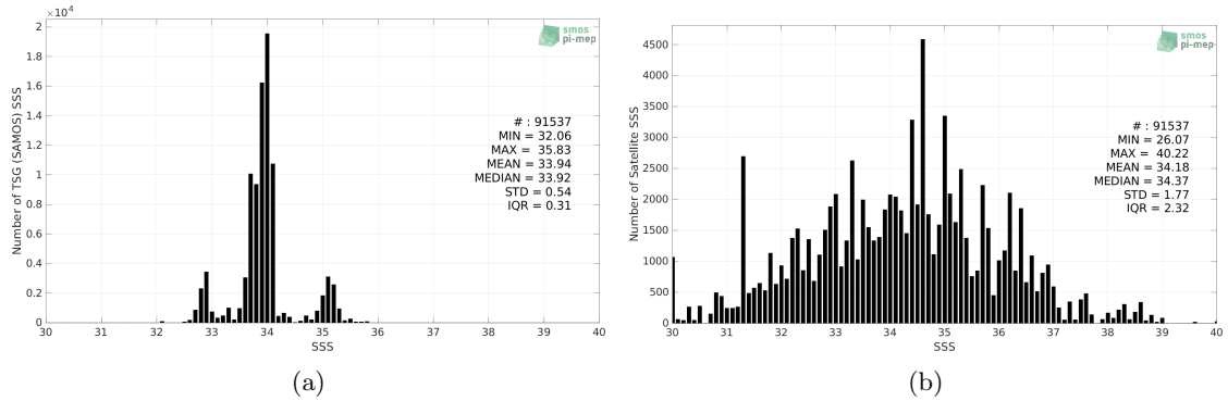
Figure 2: Histograms of SSS from TSG (SAMOS) (a) and SMOS SSS L2Q v330 - 0.25 Deg (CATDS-CPDC) (b) considering all match-up pairs per bins of 0.1 over the Roaring Forties and Furious Fifties Pi-MEP region and for the full satellite product period.
