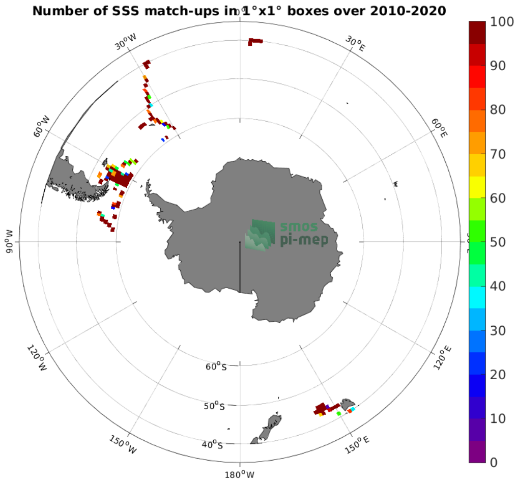
Figure 4: Number of SSS match-ups between TSG (SAMOS) SSS and the SMOS SSS L2Q v330 - 0.25 Deg (CATDS-CPDC) SSS product for the Roaring Forties and Furious Fifties Pi-MEP region over 1^\circ \times 1^\circ boxes and for the full satellite product period.
