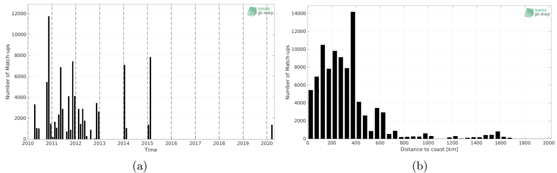
Figure 1: Number of match-ups between TSG (SAMOS) and SMOS SSS L2Q v330 - 0.25 Deg (CATDS-CPDC) SSS as a function of time (a) and as function of the distance to coast (b) over the Roaring Forties and Furious Fifties Pi-MEP region and for the full satellite product period.
