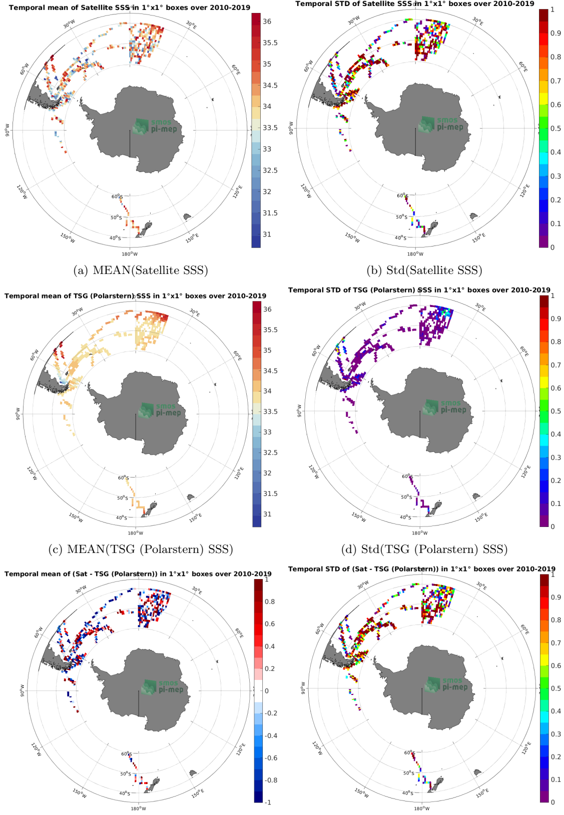
Figure 6: Temporal mean (left) and Std (right) of SSS from SMOS SSS L2Q v330 - 0.25 Deg (CATDS-CPDC) (top), TSG (Polarstern) (middle), and of \Delta SSS (Satellite - TSG (Polarstern)). Only match-up pairs are used to generate these maps.
