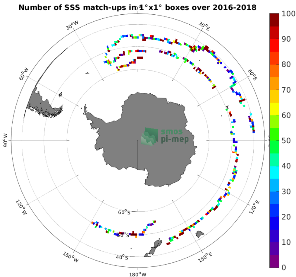
Figure 3: Number of SSS match-ups between Surface drifters SSS and the SMOS SSS L2Q v330 - 0.25 Deg (CATDS-CPDC) SSS product for the Roaring Forties and Furious Fifties Pi-MEP region over 1^\circ \times 1^\circ boxes and for the full satellite product period.
