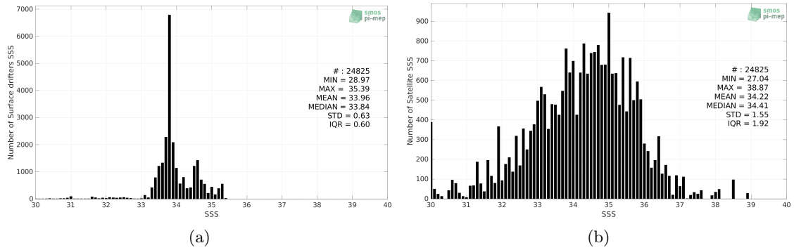
Figure 2: Histograms of SSS from Surface drifters (a) and SMOS SSS L2Q v330 - 0.25 Deg (CATDS-CPDC) (b) considering all match-up pairs per bins of 0.1 over the Roaring Forties and Furious Fifties Pi-MEP region and for the full satellite product period.
