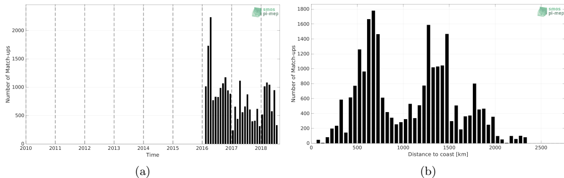
Figure 1: Number of match-ups between Surface drifters and SMOS SSS L2Q v330 - 0.25 Deg (CATDS-CPDC) SSS as a function of time (a) and as function of the distance to coast (b) over the Roaring Forties and Furious Fifties Pi-MEP region and for the full satellite product period.
