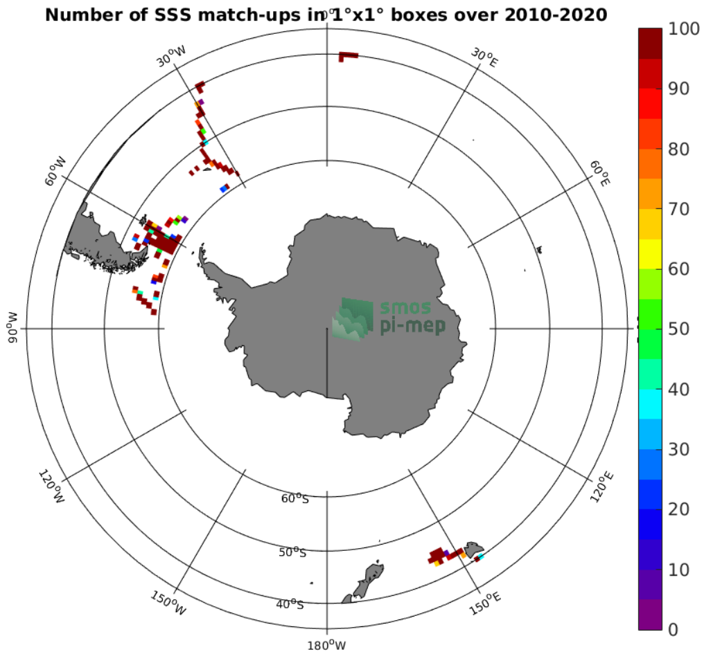
Figure 4: Number of SSS match-ups between TSG (SAMOS) SSS and the SMOS SSS L2Q v321 - 0.25 Deg (CATDS-CPDC) SSS product for the Roaring Forties and Furious Fifties Pi-MEP region over 1^\circ \times 1^\circ boxes and for the full satellite product period.
