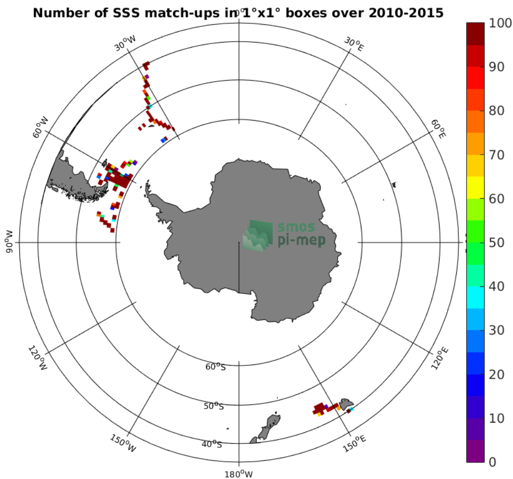
Figure 4: Number of SSS match-ups between TSG-SAMOS SSS and the SMOS L2Q v321 - 0.25 Deg (CATDS-CPDC) SSS product for the Roaring Forties and Furious Fifties Pi-MEP region over 1°x1° boxes and for the full satellite product period.
