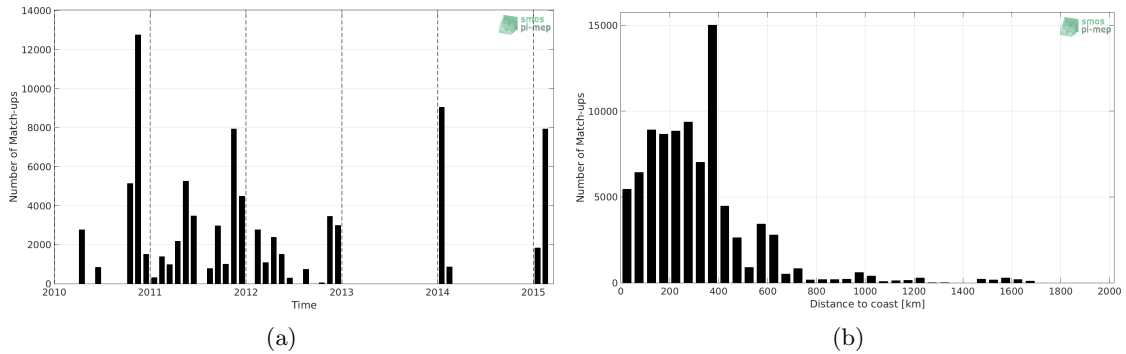
Figure 1: Number of match-ups between TSG-SAMOS and SMOS L2Q v321 - 0.25 Deg (CATDS-CPDC) SSS as a function of time (a) and as function of the distance to coast (b) over the Roaring Forties and Furious Fifties Pi-MEP region and for the full satellite product period.
