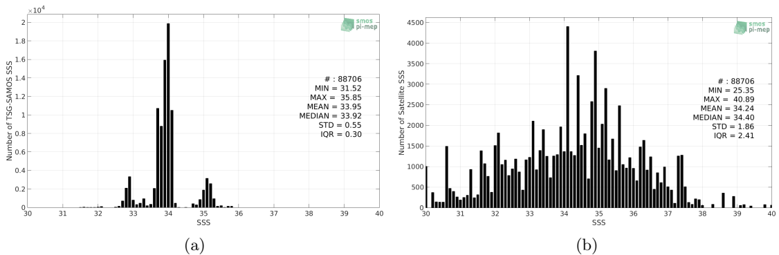
Figure 2: Histograms of SSS from TSG-SAMOS (a) and SMOS L2Q v321 - 0.25 Deg (CATDS-CPDC) (b) considering all match-up pairs per bins of 0.1 over the Roaring Forties and Furious Fifties Pi-MEP region and for the full satellite product period.
