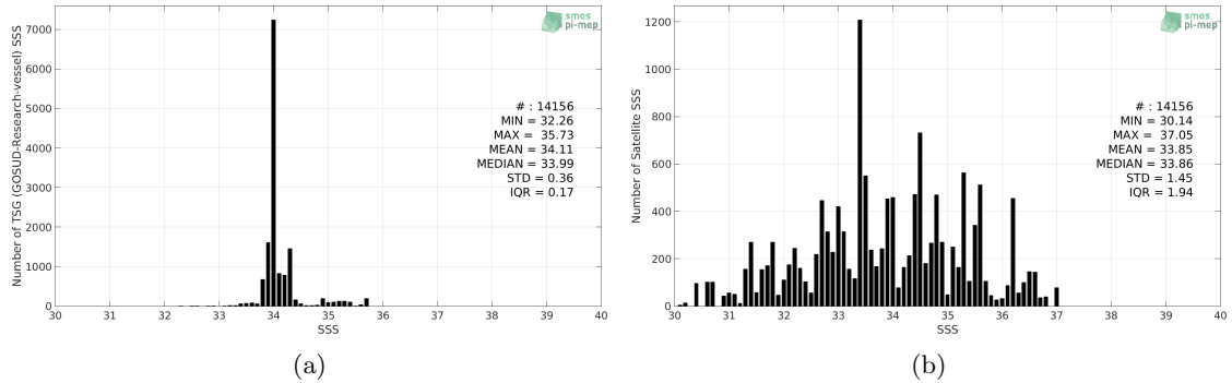
Figure 2: Histograms of SSS from TSG (GOSUD-Research-vessel) (a) and SMOS SSS L2Q v321 - 0.25 Deg (CATDS-CPDC) (b) considering all match-up pairs per bins of 0.1 over the Roaring Forties and Furious Fifties Pi-MEP region and for the full satellite product period.
