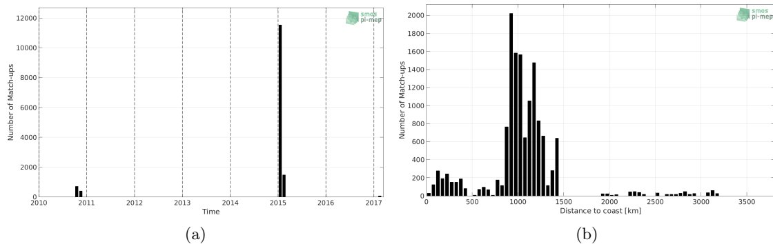
Figure 1: Number of match-ups between TSG (GOSUD-Research-vessel) and SMOS SSS L2Q v321 - 0.25 Deg (CATDS-CPDC) SSS as a function of time (a) and as function of the distance to coast (b) over the Roaring Forties and Furious Fifties Pi-MEP region and for the full satellite product period.
