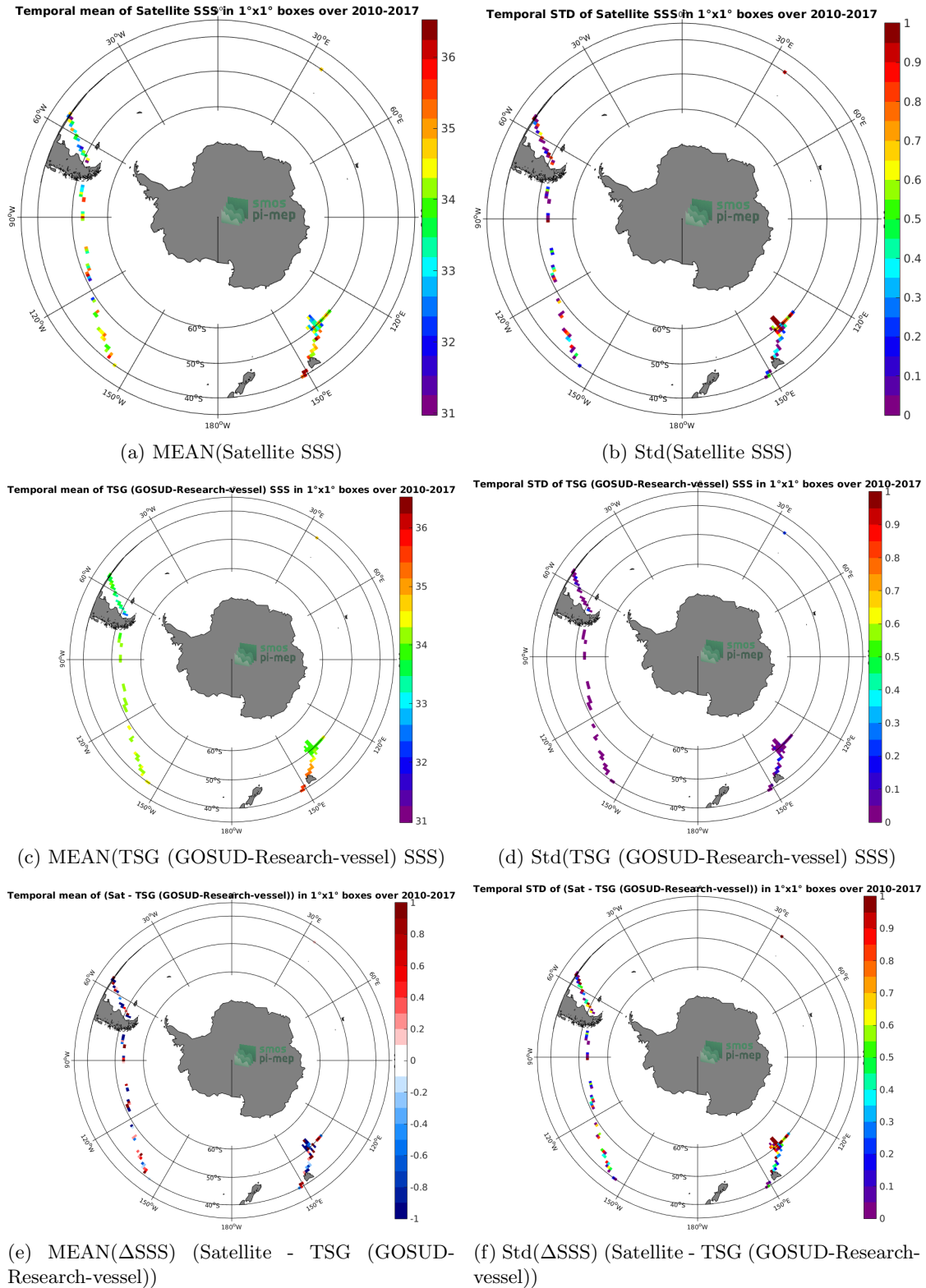
Figure 6: Temporal mean (left) and Std (right) of SSS from SMOS SSS L2Q v321 - 0.25 Deg (CATDS-CPDC) (top), TSG (GOSUD-Research-vessel) (middle), and of \Delta SSS (Satellite - TSG (GOSUD-Research-vessel)). Only match-up pairs are used to generate these maps.
