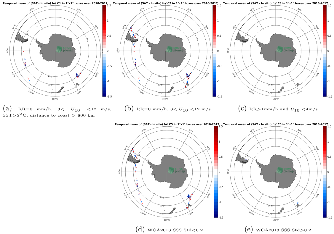
Figure 12: Temporal mean gridded over spatial boxes of size 1°x1° of \Delta SSS (SMOS SSS L2Q v321 - 0.25 Deg (CATDS-CPDC) - TSG (GOSUD-Research-vessel)) for 5 different subdatasets corresponding to: RR=0 mm/h, 3 < U_{10} < 12 m/s, SST > 5°C, distance to coast > 800 km (a), RR=0 mm/h, 3 < U_{10} < 12 m/s (b), RR > 1mm/h and U_{10} < 4 m/s (c), WOA2013 SSS Std < 0.2 (d), WOA2013 SSS Std > 0.2 (e).
