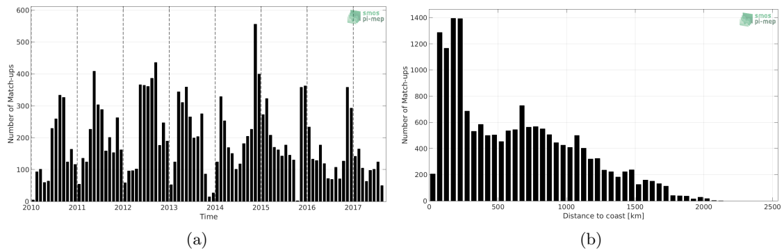
Figure 1: Number of match-ups between Marine mammals and SMOS SSS L2Q v321 - 0.25 Deg (CATDS-CPDC) SSS as a function of time (a) and as function of the distance to coast (b) over the Roaring Forties and Furious Fifties Pi-MEP region and for the full satellite product period.
