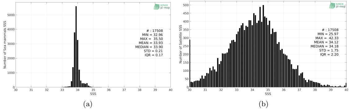
Figure 2: Histograms of SSS from Marine mammals (a) and SMOS SSS L2Q v321 - 0.25 Deg (CATDS-CPDC) (b) considering all match-up pairs per bins of 0.1 over the Roaring Forties and Furious Fifties Pi-MEP region and for the full satellite product period.
