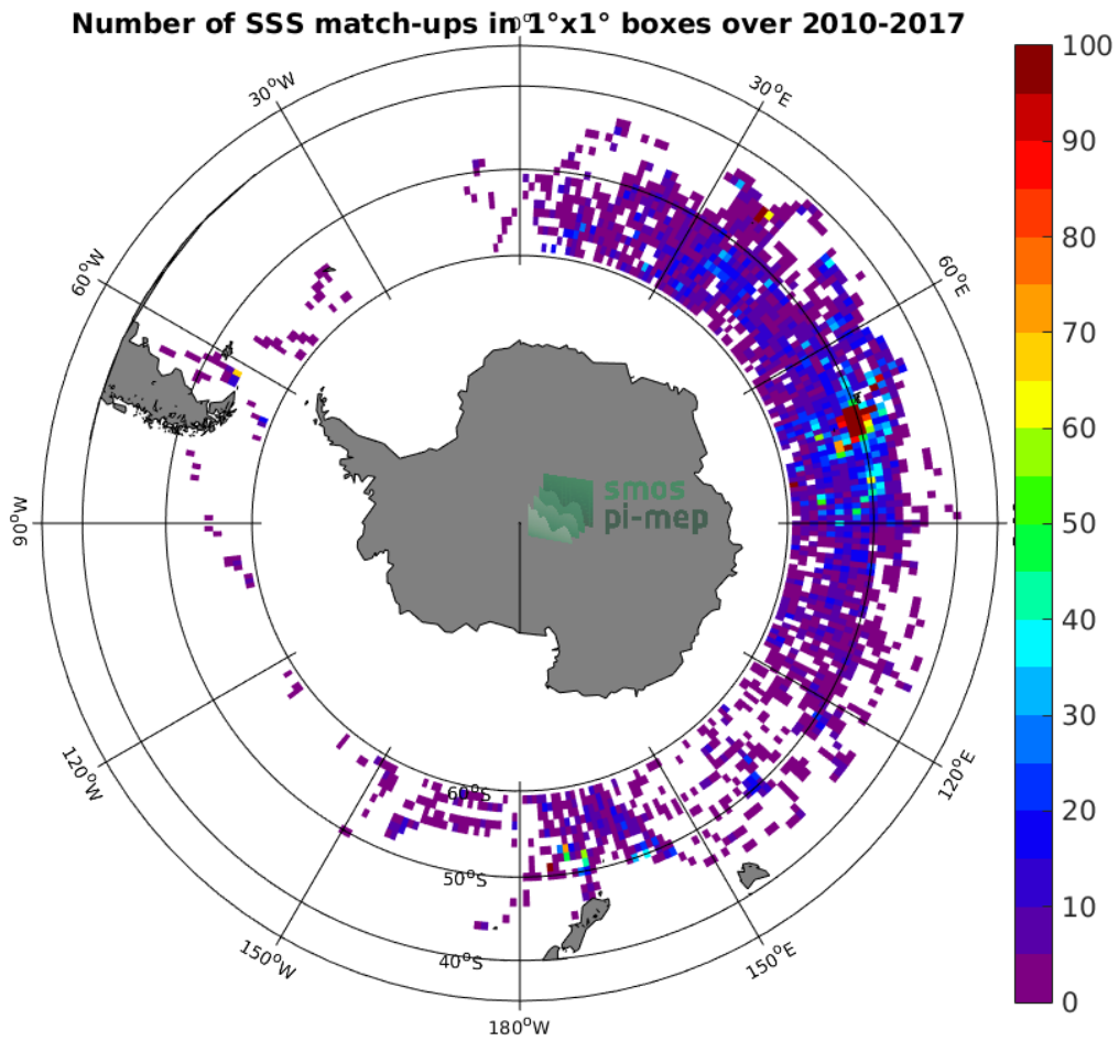
Figure 4: Number of SSS match-ups between Marine mammals SSS and the SMOS SSS L2Q v321 - 0.25 Deg (CATDS-CPDC) SSS product for the Roaring Forties and Furious Fifties Pi-MEP region over 1^\circ \times 1^\circ boxes and for the full satellite product period.
