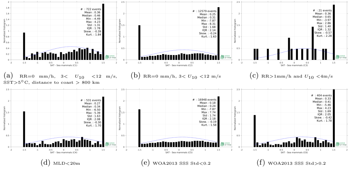
Figure 13: Normalized histogram of \Delta SSS (SMOS SSS L2Q v321 - 0.25 Deg (CATDS-CPDC) - Marine mammals) for 6 different subdatasets corresponding to: RR=0 mm/h, 3 < U_{10} < 12 m/s, SST>5°C, distance to coast > 800 km (a), RR=0 mm/h, 3 < U_{10} < 12 m/s (b), RR>1mm/h and U_{10} < 4 m/s (c), MLD<20m (d), WOA2013 SSS Std<0.2 (e), WOA2013 SSS Std>0.2 (f).
