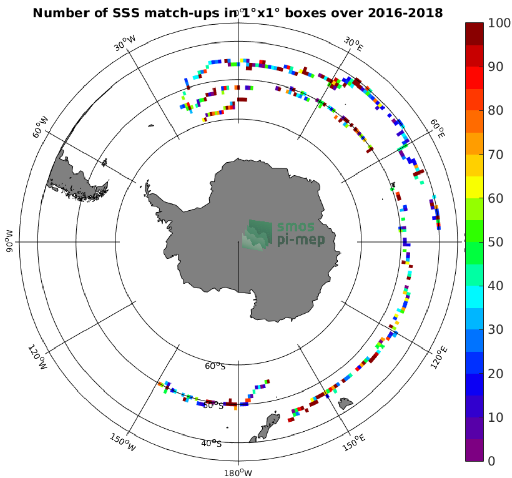
Figure 3: Number of SSS match-ups between Surface drifters SSS and the SMOS L2Q v321 - 0.25 Deg (CATDS-CPDC) SSS product for the Roaring Forties and Furious Fifties Pi-MEP region over 1°x1° boxes and for the full satellite product period.
