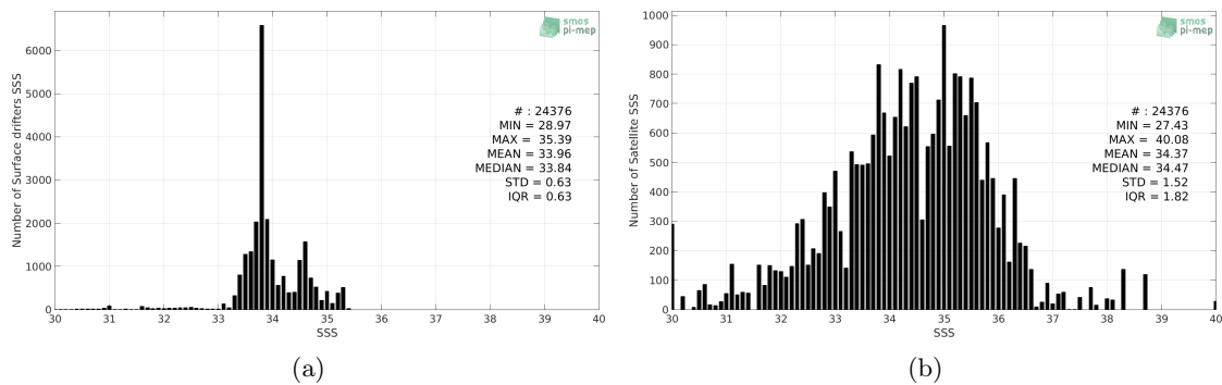
Figure 2: Histograms of SSS from Surface drifters (a) and SMOS L2Q v321 - 0.25 Deg (CATDS-CPDC) (b) considering all match-up pairs per bins of 0.1 over the Roaring Forties and Furious Fifties Pi-MEP region and for the full satellite product period.
