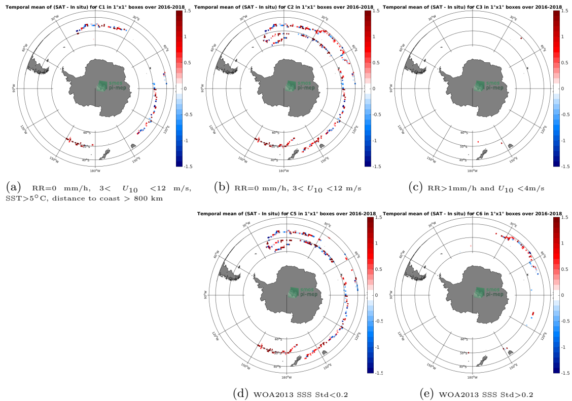
Figure 11: Temporal mean gridded over spatial boxes of size 1^{\circ}\times 1^{\circ} of \Delta\text{SSS} (SMOS L2Q v321 - 0.25 Deg (CATDS-CPDC) - Surface drifters) for 5 different subdatasets corresponding to:RR=0 mm/h, 3 < U_{10} < 12 m/s, SST >5^{\circ}\text{C} , distance to coast > 800 km (a), RR=0 mm/h, 3 < U_{10} < 12 m/s (b), RR >1 mm/h and U_{10} < 4 m/s (c), WOA2013 SSS Std <0.2 (d), WOA2013 SSS Std >0.2 (e).
