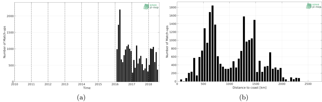
Figure 1: Number of match-ups between Surface drifters and SMOS L2Q v321 - 0.25 Deg (CATDS-CPDC) SSS as a function of time (a) and as function of the distance to coast (b) over the Roaring Forties and Furious Fifties Pi-MEP region and for the full satellite product period.
