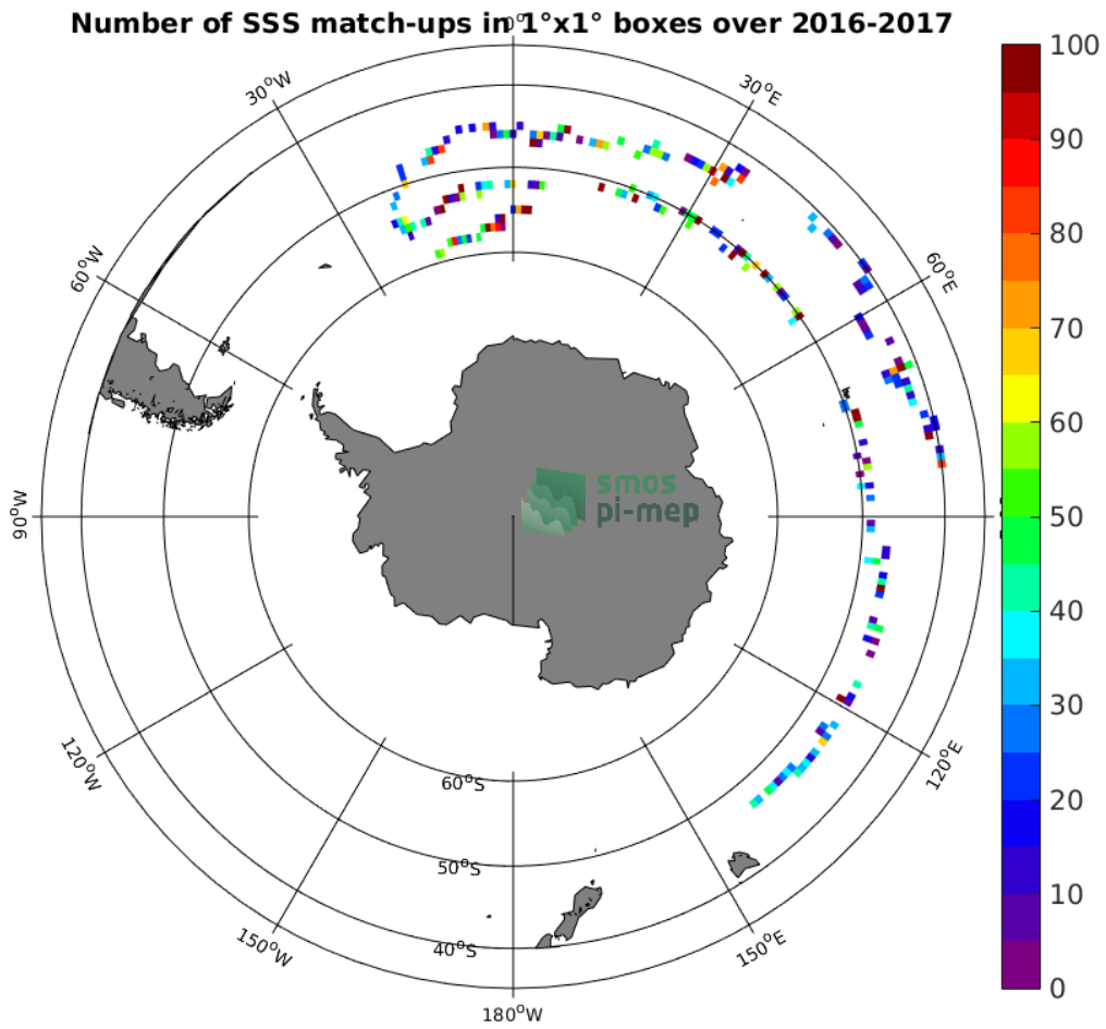
Figure 3: Number of SSS match-ups between Surface drifters SSS and the SMOS-L3-CATDS-CPDC-V321-L2Q SSS product for the Roaring Forties and Furious Fifties Pi-MEP region over 1°x1° boxes and for the full satellite product period.
