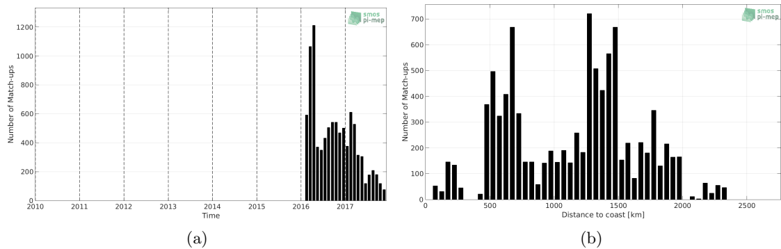
Figure 1: Number of match-ups between Surface drifters and SMOS-L3-CATDS-CPDC-V321-L2Q SSS as a function of time (a) and as function of the distance to coast (b) over the Roaring Forties and Furious Fifties Pi-MEP region and for the full satellite product period.
