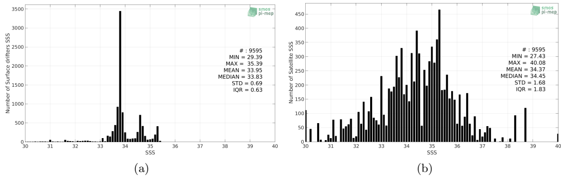
Figure 2: Histograms of SSS from Surface drifters (a) and SMOS-L3-CATDS-CPDC-V321-L2Q (b) considering all match-up pairs per bins of 0.1 over the Roaring Forties and Furious Fifties Pi-MEP region and for the full satellite product period.
