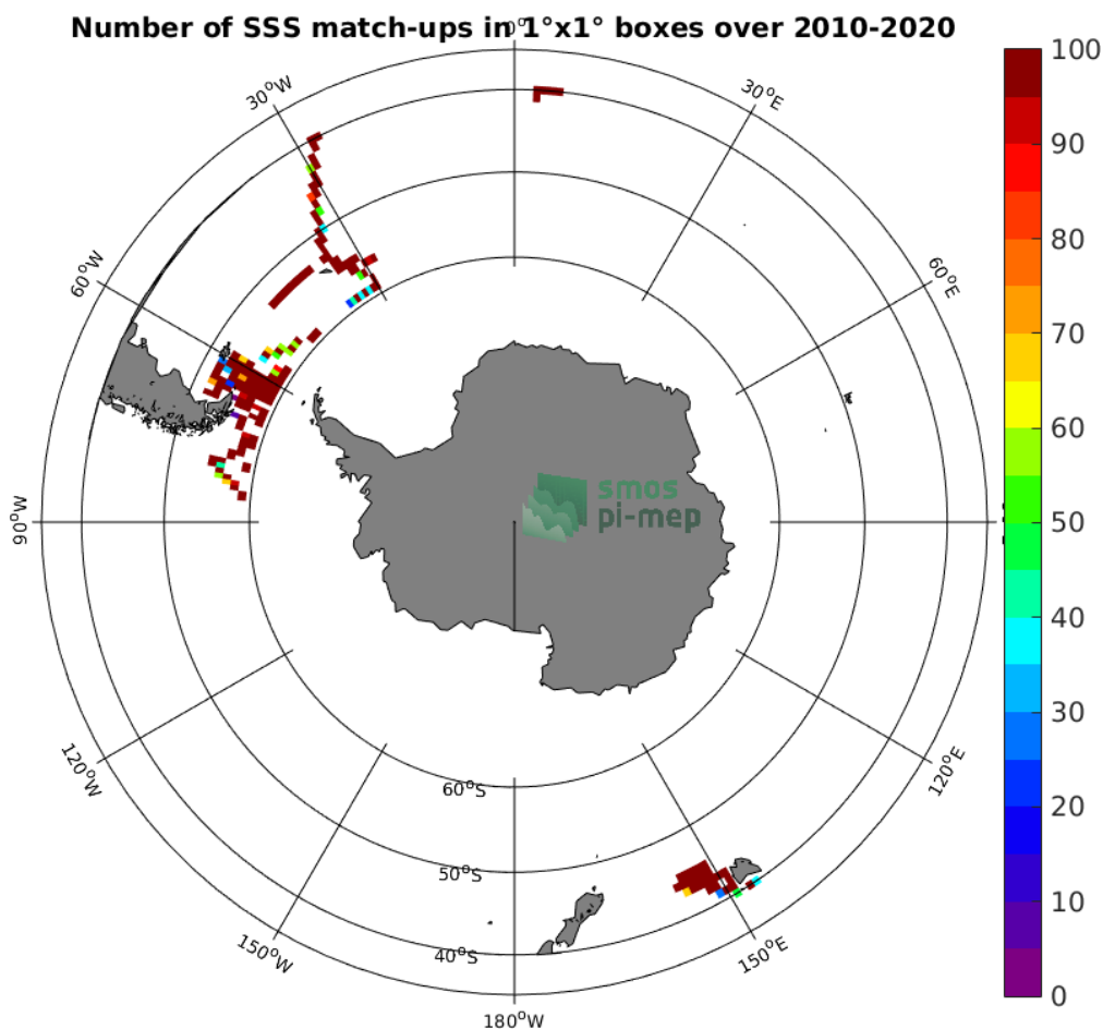
Figure 4: Number of SSS match-ups between TSG (SAMOS) SSS and the SMOS SSS L3 v317 - Monthly - 25 km (CATDS-CPDC) SSS product for the Roaring Forties and Furious Fifties Pi-MEP region over 1°x1° boxes and for the full satellite product period.
