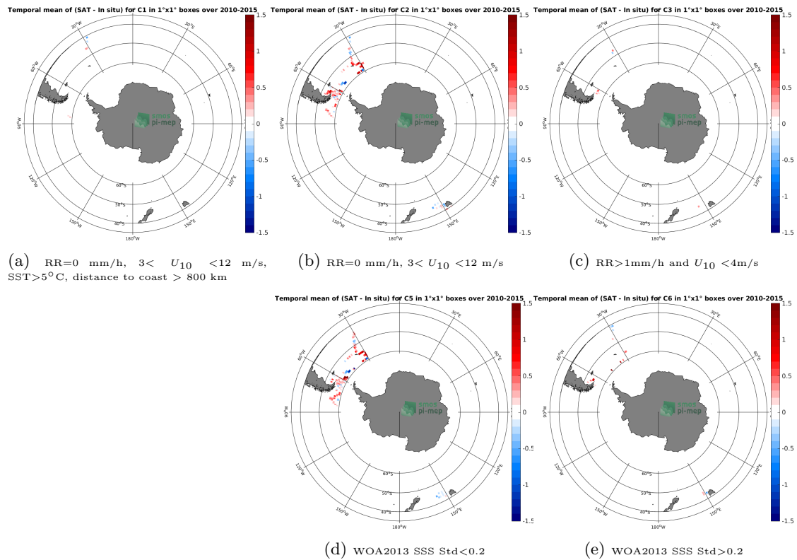
Figure 12: Temporal mean gridded over spatial boxes of size 1^{\circ}\times 1^{\circ} of \Delta\text{SSS} (SMOS L3 v317 - Monthly - 25 km (CATDS-CPDC) - TSG-SAMOS) for 5 different subdatasets corresponding to:RR=0 mm/h, 3 < U_{10} < 12 m/s, SST > 5^{\circ}\text{C} , distance to coast > 800 km (a), RR=0 mm/h, 3 < U_{10} < 12 m/s (b), RR > 1 mm/h and U_{10} < 4 m/s (c), WOA2013 SSS Std < 0.2 (d), WOA2013 SSS Std > 0.2 (e).
