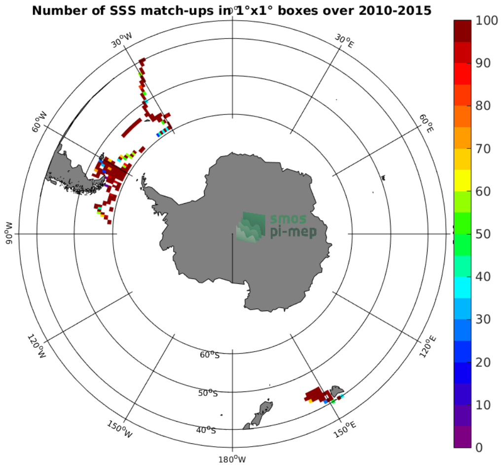
Figure 4: Number of SSS match-ups between TSG-SAMOS SSS and the SMOS L3 v317 - Monthly - 25 km (CATDS-CPDC) SSS product for the Roaring Forties and Furious Fifties Pi-MEP region over 1°x1° boxes and for the full satellite product period.
