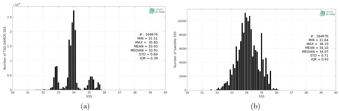
Figure 2: Histograms of SSS from TSG-SAMOS (a) and SMOS L3 v317 - Monthly - 25 km (CATDS-CPDC) (b) considering all match-up pairs per bins of 0.1 over the Roaring Forties and Furious Fifties Pi-MEP region and for the full satellite product period.
