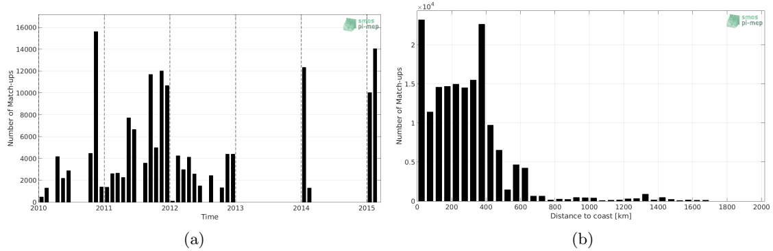
Figure 1: Number of match-ups between TSG-SAMOS and SMOS L3 v317 - Monthly - 25 km (CATDS-CPDC) SSS as a function of time (a) and as function of the distance to coast (b) over the Roaring Forties and Furious Fifties Pi-MEP region and for the full satellite product period.
