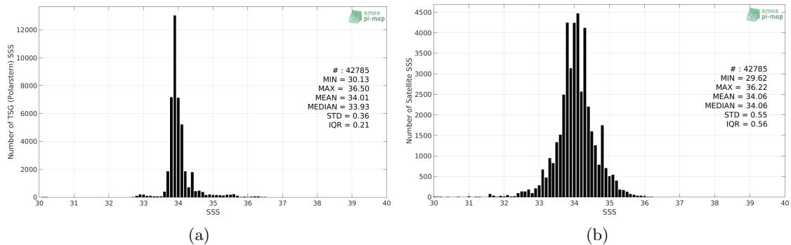
Figure 2: Histograms of SSS from TSG (Polarstern) (a) and SMOS SSS L3 v317 - Monthly - 25 km (CATDS-CPDC) (b) considering all match-up pairs per bins of 0.1 over the Roaring Forties and Furious Fifties Pi-MEP region and for the full satellite product period.
