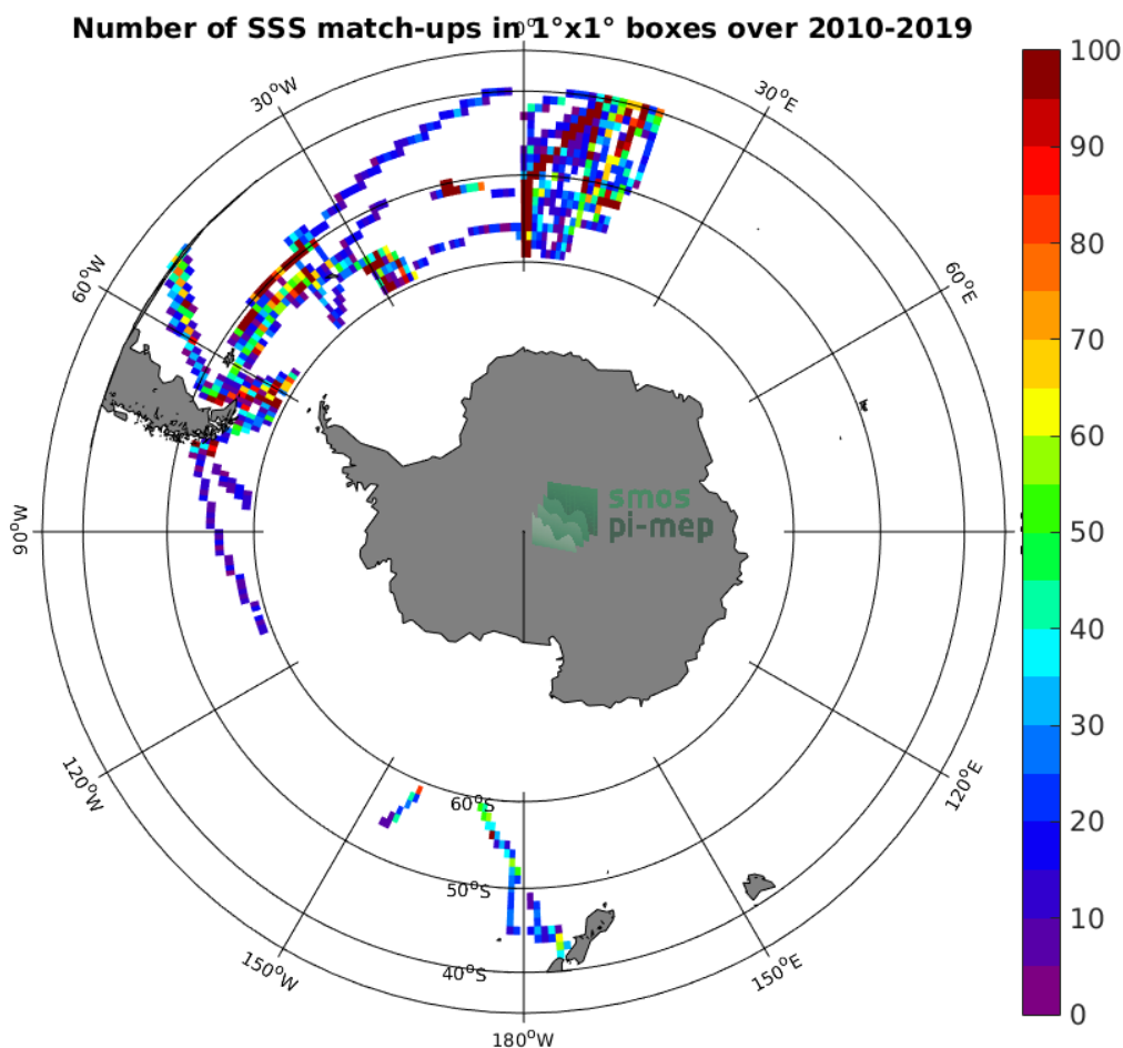
Figure 4: Number of SSS match-ups between TSG (Polarstern) SSS and the SMOS SSS L3 v317 - Monthly - 25 km (CATDS-CPDC) SSS product for the Roaring Forties and Furious Fifties Pi-MEP region over 1°x1° boxes and for the full satellite product period.
