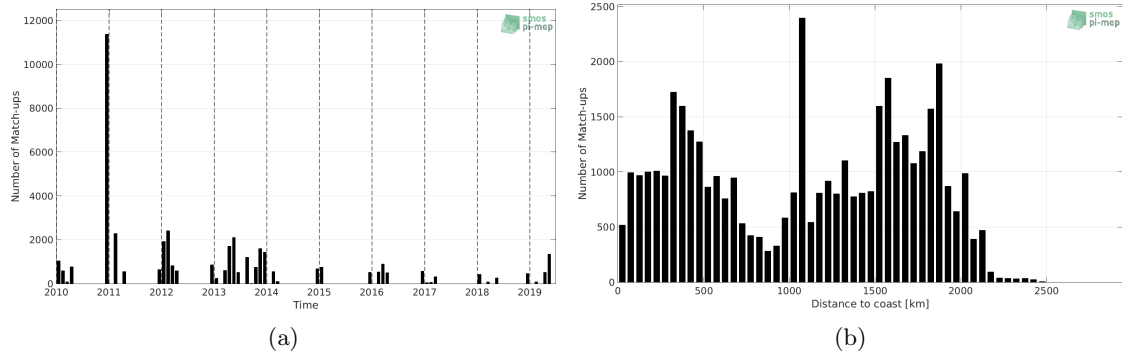
Figure 1: Number of match-ups between TSG (Polarstern) and SMOS SSS L3 v317 - Monthly - 25 km (CATDS-CPDC) SSS as a function of time (a) and as function of the distance to coast (b) over the Roaring Forties and Furious Fifties Pi-MEP region and for the full satellite product period.
