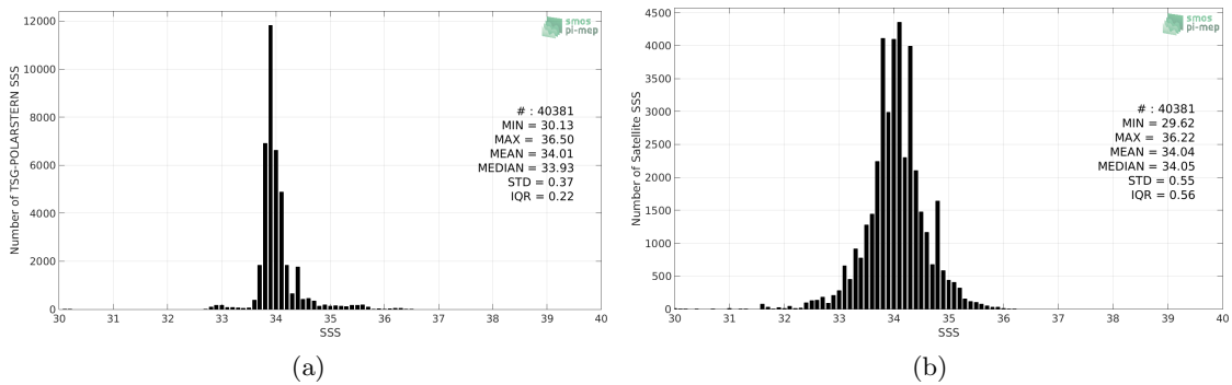
Figure 2: Histograms of SSS from TSG-POLARSTERN (a) and SMOS-L3-CATDS-CPDC-V317-MONTHLY-25KM (b) considering all match-up pairs per bins of 0.1 over the Roaring Forties and Furious Fifties Pi-MEP region and for the full satellite product period.
