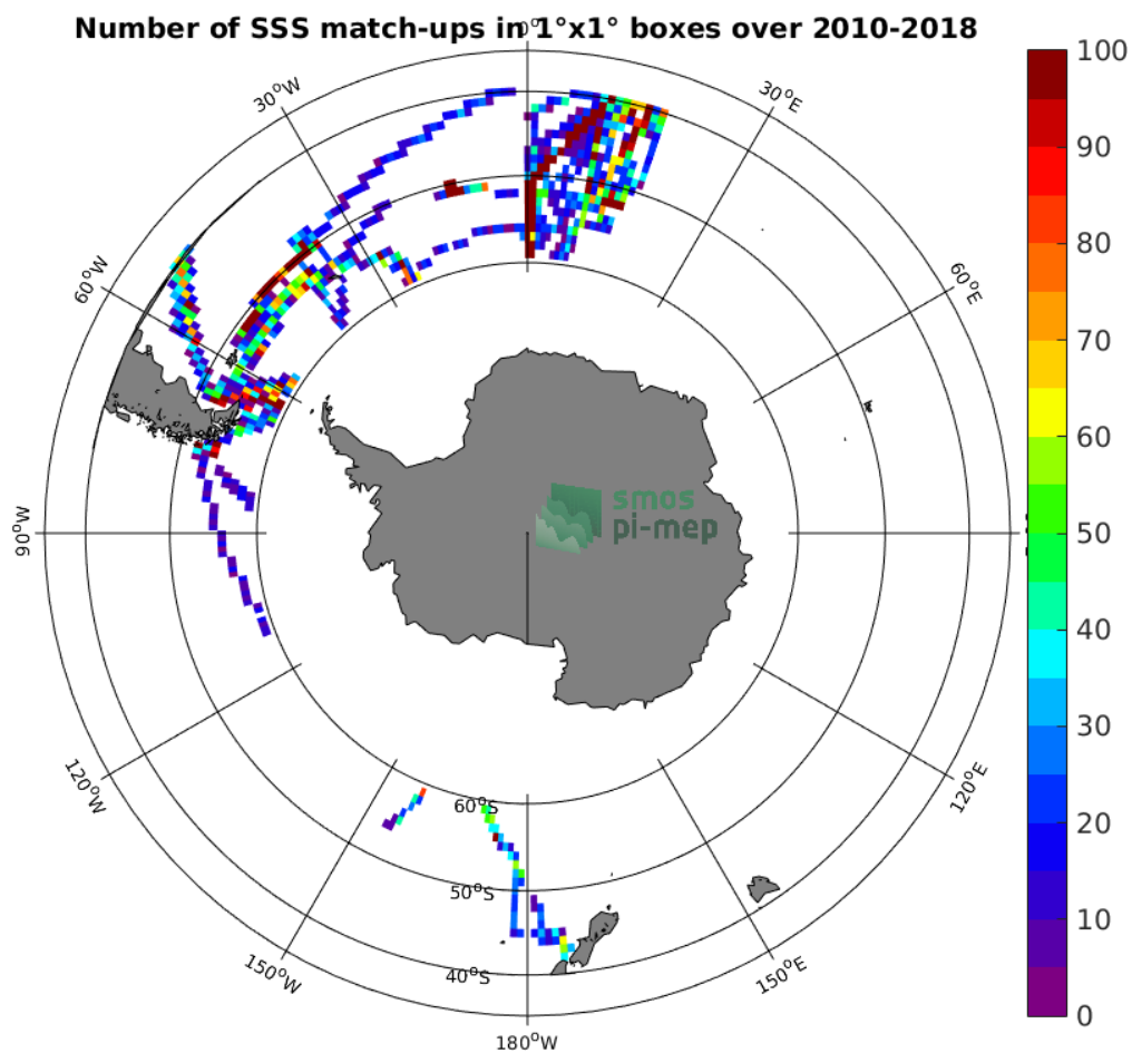
Figure 4: Number of SSS match-ups between TSG-POLARSTERN SSS and the SMOS-L3-CATDS-CPDC-V317-MONTHLY-25KM SSS product for the Roaring Forties and Furious Fifties Pi-MEP region over 1^{\circ} \times 1^{\circ} boxes and for the full satellite product period.
