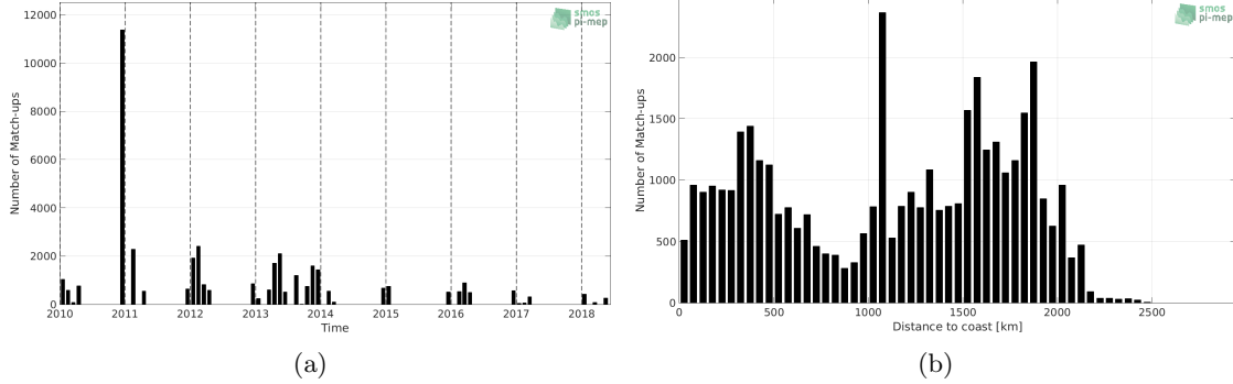
Figure 1: Number of match-ups between TSG-POLARSTERN and SMOS-L3-CATDS-CPDC-V317-MONTHLY-25KM SSS as a function of time (a) and as function of the distance to coast (b) over the Roaring Forties and Furious Fifties Pi-MEP region and for the full satellite product period.
