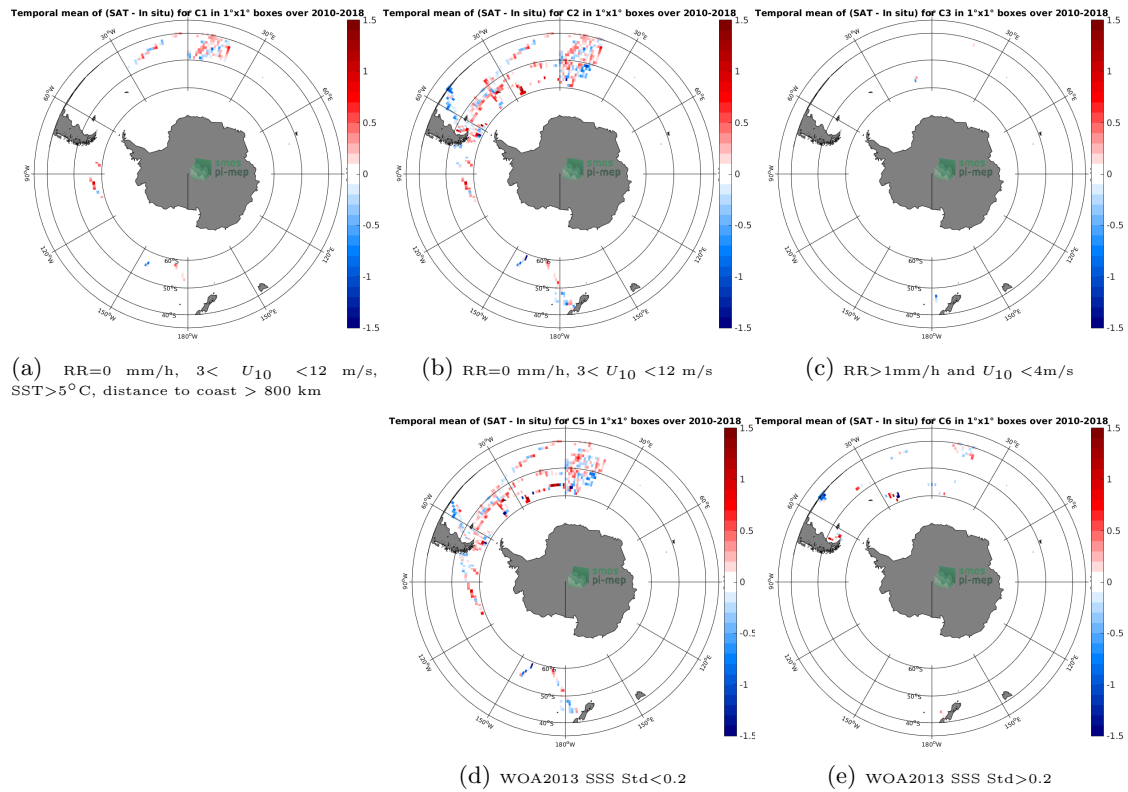
Figure 12: Temporal mean gridded over spatial boxes of size 1°x1° of \Delta SSS (SMOS-L3-CATDS-CPDC-V317-MONTHLY-25KM - TSG-POLARSTERN) for 5 different subdatasets corresponding to:RR=0 mm/h, 3 < U_{10} < 12 m/s, SST>5°C, distance to coast > 800 km (a), RR=0 mm/h, 3 < U_{10} < 12 m/s (b), RR>1mm/h and U_{10} < 4 m/s (c), WOA2013 SSS Std<0.2 (d), WOA2013 SSS Std>0.2 (e).
