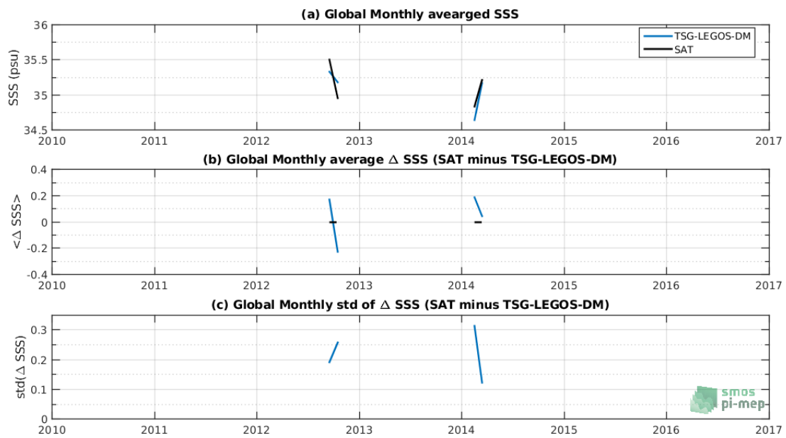
Figure 7: Time series of the monthly averaged mean SSS (top), mean \Delta SSS (Satellite - TSG-LEGOS-DM) and Std of \Delta SSS (Satellite - TSG-LEGOS-DM) over the Roaring Forties and Furious Fifties Pi-MEP region considering all match-ups collected by the Pi-MEP platform.
