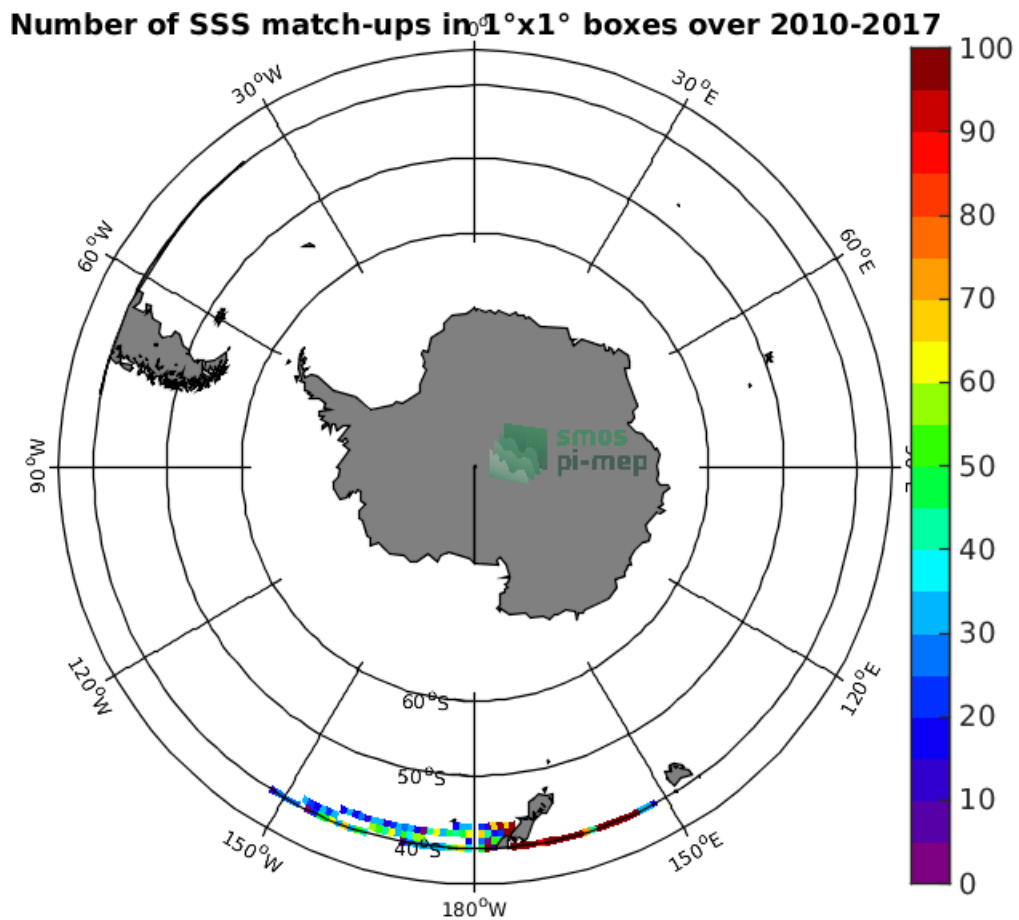
Figure 4: Number of SSS match-ups between TSG-LEGOS-DM SSS and the SMOS-L3-CATDS-CPDC-V317-MONTHLY-25KM SSS product for the Roaring Forties and Furious Fifties Pi-MEP region over 1°x1° boxes and for the full satellite product period.
