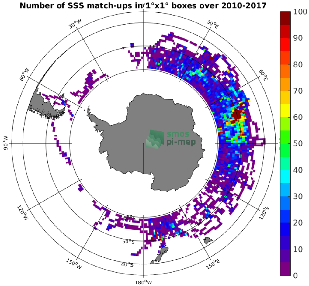
Figure 4: Number of SSS match-ups between Sea mammals SSS and the SMOS SSS L3 v317 - Monthly - 25 km (CATDS-CPDC) SSS product for the Roaring Forties and Furious Fifties Pi-MEP region over 1^\circ \times 1^\circ boxes and for the full satellite product period.
