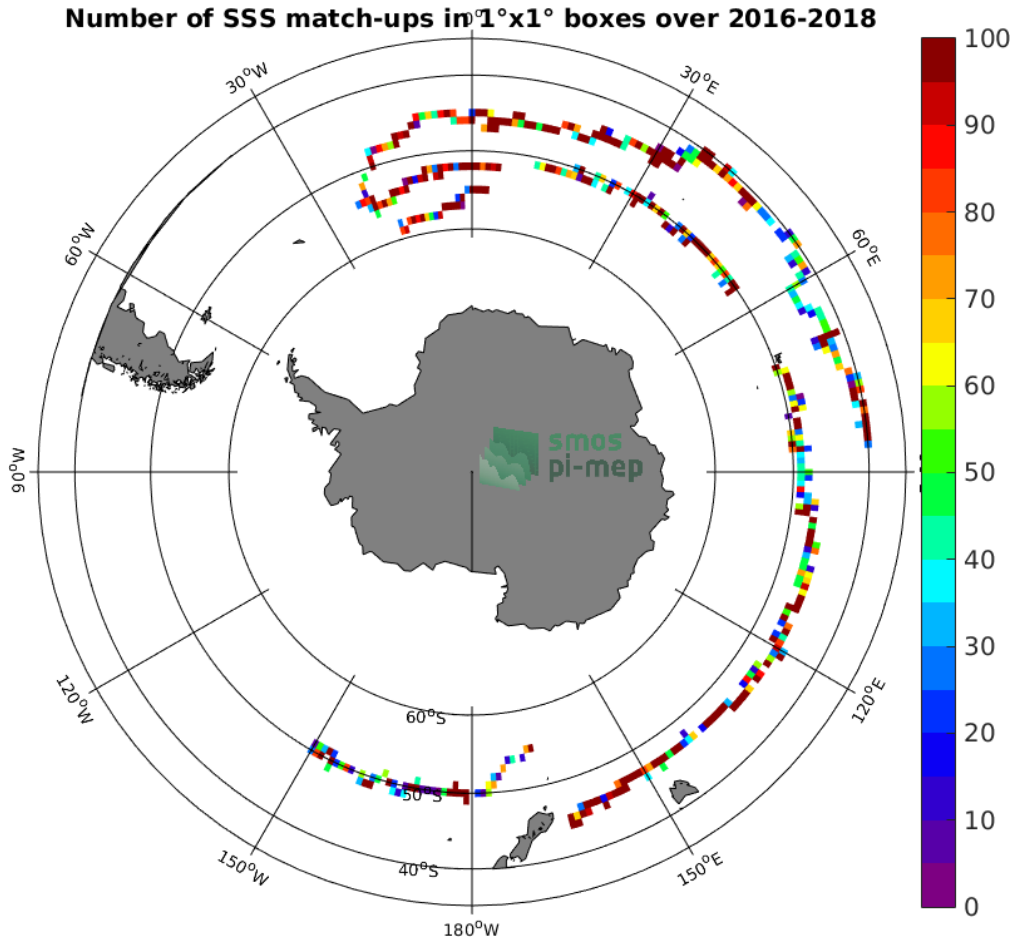
Figure 3: Number of SSS match-ups between Surface drifters SSS and the SMOS SSS L3 v317 - Monthly - 25 km (CATDS-CPDC) SSS product for the Roaring Forties and Furious Fifties Pi-MEP region over 1°x1° boxes and for the full satellite product period.
