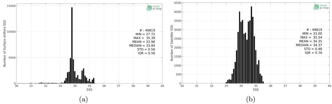
Figure 2: Histograms of SSS from Surface drifters (a) and SMOS L3 v317 - Monthly - 25 km (CATDS-CPDC) (b) considering all match-up pairs per bins of 0.1 over the Roaring Forties and Furious Fifties Pi-MEP region and for the full satellite product period.
