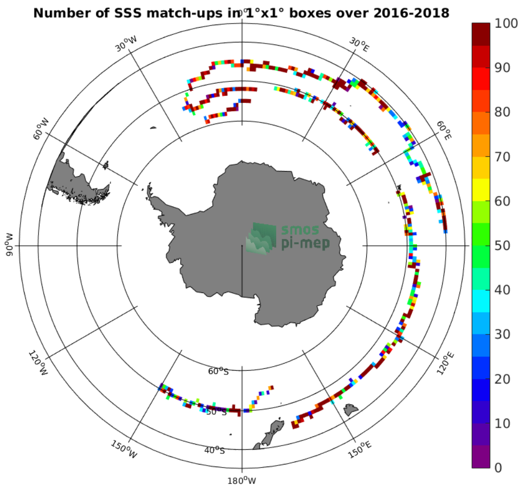
Figure 3: Number of SSS match-ups between Surface drifters SSS and the SMOS L3 v317 - Monthly - 25 km (CATDS-CPDC) SSS product for the Roaring Forties and Furious Fifties Pi-MEP region over 1°x1° boxes and for the full satellite product period.
