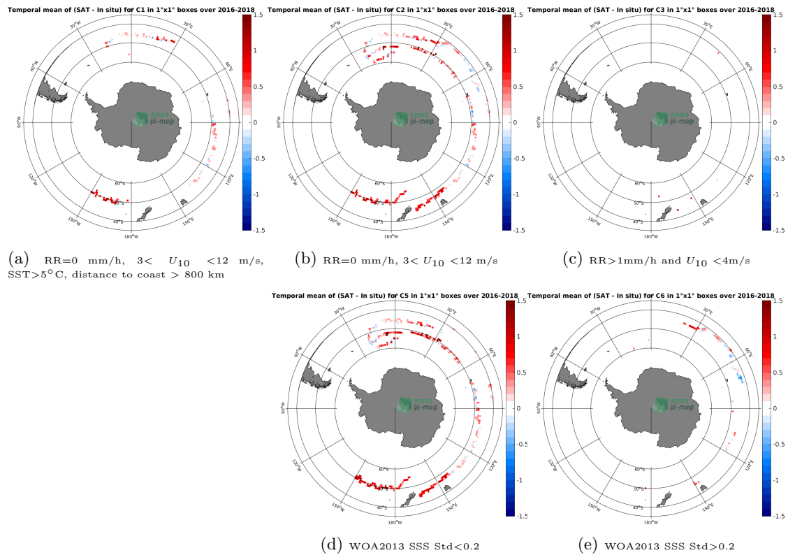
Figure 11: Temporal mean gridded over spatial boxes of size 1^{\circ}\times 1^{\circ} of \Delta\text{SSS} (SMOS L3 v317 - Monthly - 25 km (CATDS-CPDC) - Surface drifters) for 5 different subdatasets corresponding to: RR=0 mm/h, 3 < U_{10} < 12 m/s, SST > 5^{\circ}\text{C} , distance to coast > 800 km (a), RR=0 mm/h, 3 < U_{10} < 12 m/s (b), RR > 1 mm/h and U_{10} < 4 m/s (c), WOA2013 SSS Std < 0.2 (d), WOA2013 SSS Std > 0.2 (e).
