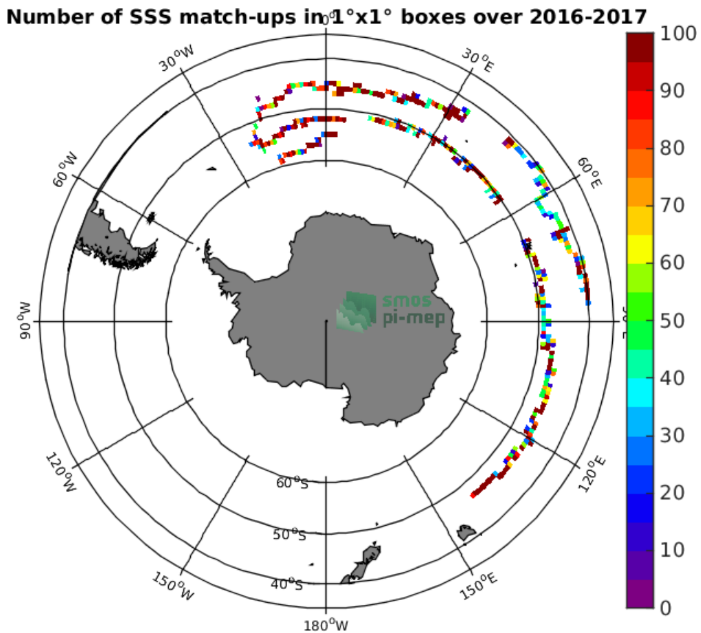
Figure 3: Number of SSS match-ups between Surface drifters SSS and the SMOS-L3-CATDS-CPDC-V317-MONTHLY-25KM SSS product for the Roaring Forties and Furious Fifties Pi-MEP region over 1°x1° boxes and for the full satellite product period.
