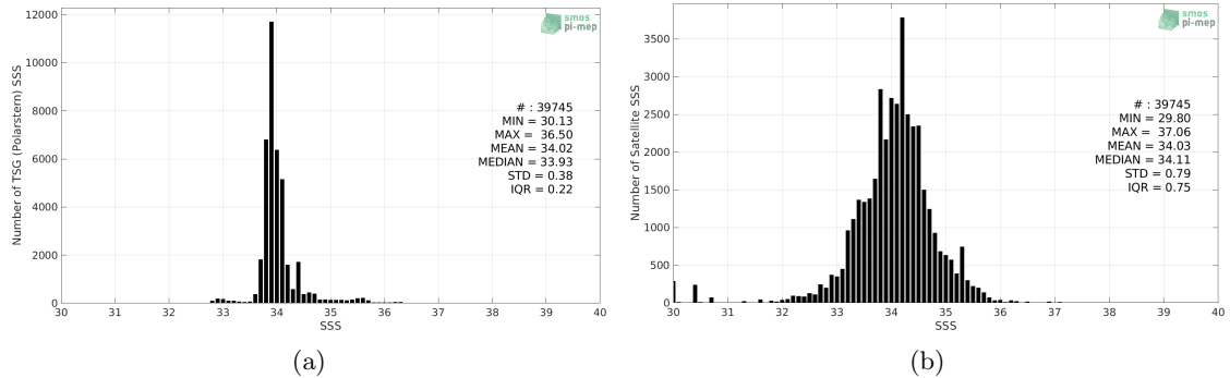
Figure 2: Histograms of SSS from TSG (Polarstern) (a) and SMOS SSS L3 v317 - 10 Days - 25 km (CATDS-CPDC) (b) considering all match-up pairs per bins of 0.1 over the Roaring Forties and Furious Fifties Pi-MEP region and for the full satellite product period.
