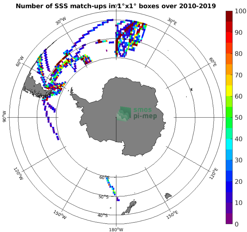
Figure 4: Number of SSS match-ups between TSG (Polarstern) SSS and the SMOS SSS L3 v317 - 10 Days - 25 km (CATDS-CPDC) SSS product for the Roaring Forties and Furious Fifties Pi-MEP region over 1^\circ \times 1^\circ boxes and for the full satellite product period.
