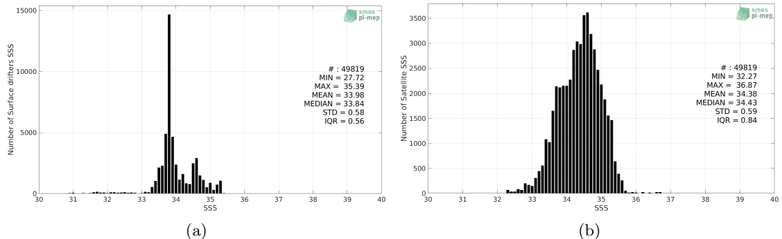
Figure 2: Histograms of SSS from Surface drifters (a) and SMOS SSS L3 v317 - 10 Days - 25 km (CATDS-CPDC) (b) considering all match-up pairs per bins of 0.1 over the Roaring Forties and Furious Fifties Pi-MEP region and for the full satellite product period.
