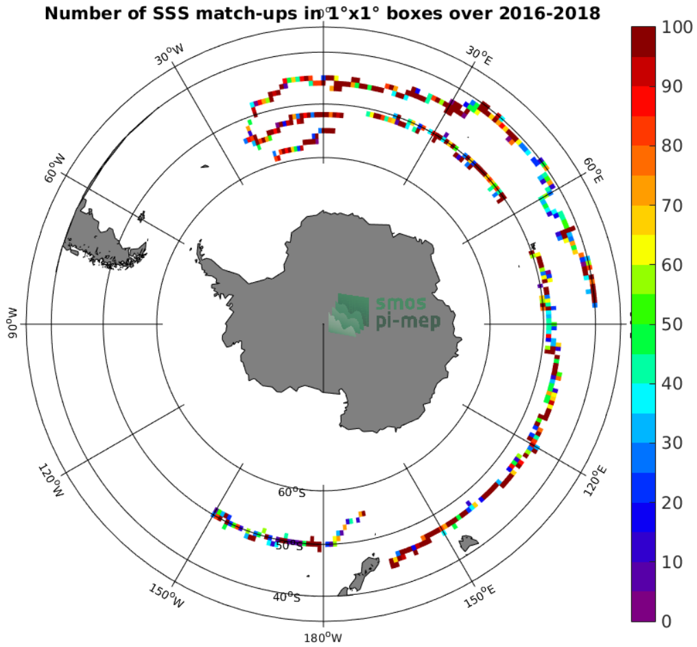
Figure 3: Number of SSS match-ups between Surface drifters SSS and the SMOS L3 v317 - 10 Days - 25 km (CATDS-CPDC) SSS product for the Roaring Forties and Furious Fifties Pi-MEP region over 1°x1° boxes and for the full satellite product period.
