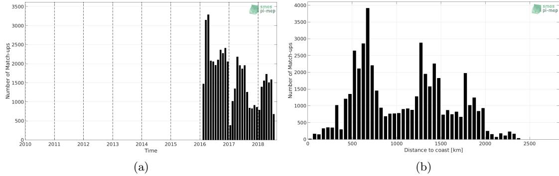
Figure 1: Number of match-ups between Surface drifters and SMOS L3 v317 - 10 Days - 25 km (CATDS-CPDC) SSS as a function of time (a) and as function of the distance to coast (b) over the Roaring Forties and Furious Fifties Pi-MEP region and for the full satellite product period.
