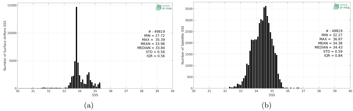
Figure 2: Histograms of SSS from Surface drifters (a) and SMOS L3 v317 - 10 Days - 25 km (CATDS-CPDC) (b) considering all match-up pairs per bins of 0.1 over the Roaring Forties and Furious Fifties Pi-MEP region and for the full satellite product period.
