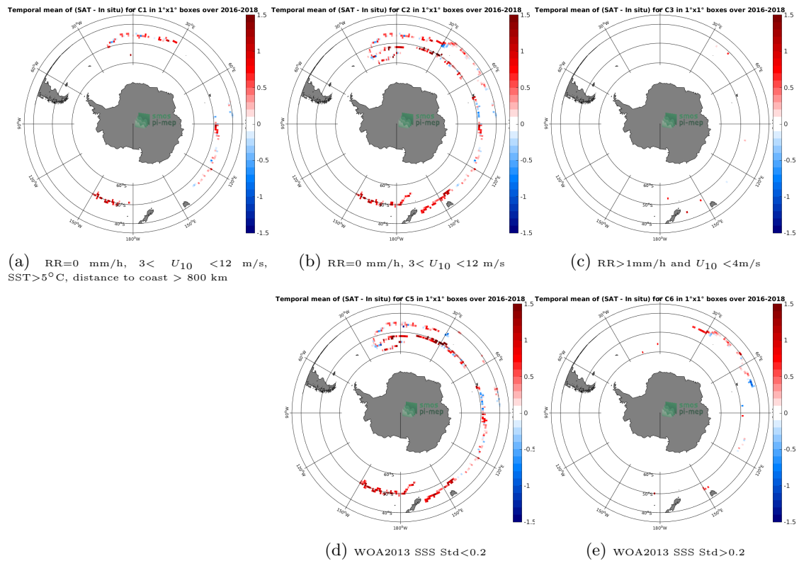
Figure 11: Temporal mean gridded over spatial boxes of size 1^{\circ}\times 1^{\circ} of \Delta\text{SSS} (SMOS L3 v317 - 10 Days - 25 km (CATDS-CPDC) - Surface drifters) for 5 different subdatasets corresponding to:RR=0 mm/h, 3 < U_{10} < 12 m/s, SST > 5^{\circ}\text{C} , distance to coast > 800 km (a), RR=0 mm/h, 3 < U_{10} < 12 m/s (b), RR > 1 mm/h and U_{10} < 4 m/s (c), WOA2013 SSS Std < 0.2 (d), WOA2013 SSS Std > 0.2 (e).
