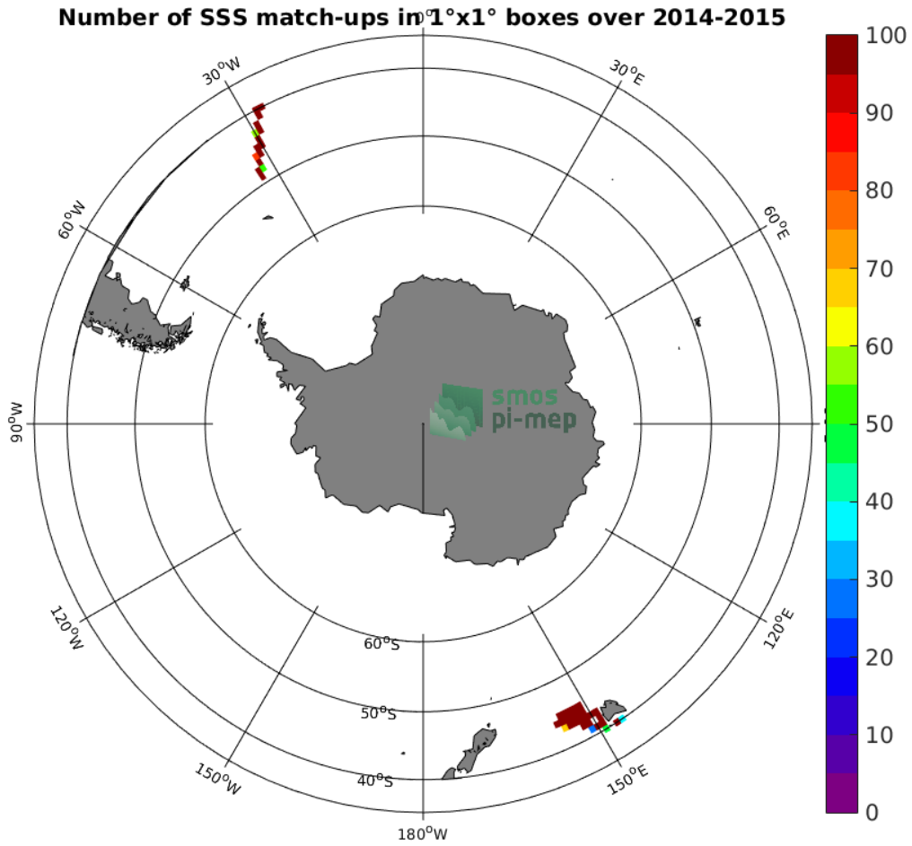
Figure 4: Number of SSS match-ups between TSG-SAMOS SSS and the SMOS-L3-CATDS-CPDC-V3-MONTHLY-25KM SSS product for the Roaring Forties and Furious Fifties Pi-MEP region over 1°x1° boxes and for the full satellite product period.
