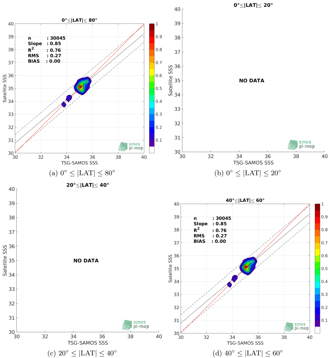
Figure 9: Contour maps of the concentration of SMOS-L3-CATDS-CPDC-V3-MONTHLY-25KM SSS (y-axis) versus TSG-SAMOS SSS (x-axis) at match-up pairs for different latitude bands. For each plot, the red line shows x=y . The black thin and dashed lines indicate a linear fit through the data cloud and the \pm 95\% confidence levels, respectively. The number match-up pairs n , the slope and R^2 coefficient of the linear fit, the root mean square (RMS) and the mean bias between satellite and in situ data are indicated for each latitude band in each plots.
