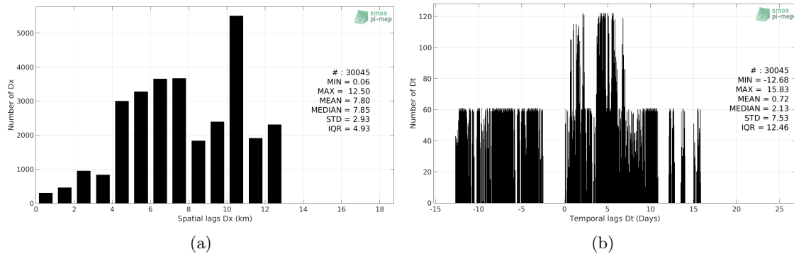
Figure 5: Histograms of the spatial (a) and temporal (b) lags between the time of the TSG-SAMOS measurements and the date of the corresponding SMOS-L3-CATDS-CPDC-V3-MONTHLY-25KM SSS product.
