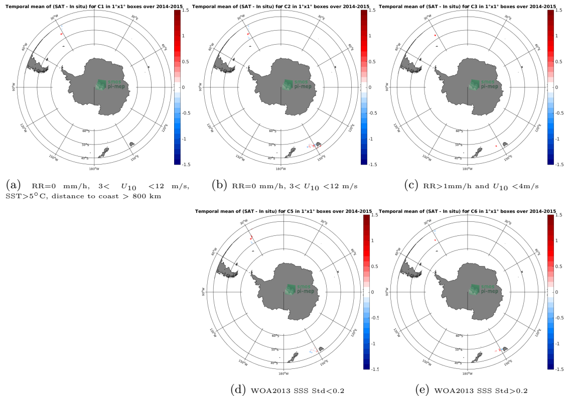
Figure 12: Temporal mean gridded over spatial boxes of size 1^\circ \times 1^\circ of \Delta SSS (SMOS-L3-CATDS-CPDC-V3-MONTHLY-25KM - TSG-SAMOS) for 5 different subdatasets corresponding to:RR=0 mm/h, 3 < U_{10} < 12 m/s, SST >5^\circ C, distance to coast > 800 km (a), RR=0 mm/h, 3 < U_{10} < 12 m/s (b), RR >1 mm/h and U_{10} < 4 m/s (c), WOA2013 SSS Std <0.2 (d), WOA2013 SSS Std >0.2 (e).
