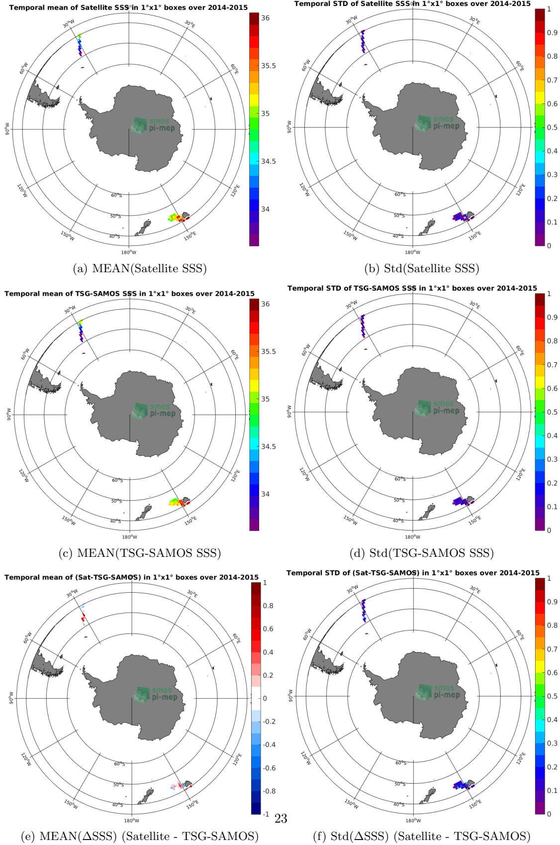
Figure 6: Temporal mean (left) and Std (right) of SSS from SMOS-L3-CATDS-CPDC-V3-MONTHLY-25KM (top), TSG-SAMOS (middle), and of \Delta SSS (Satellite - TSG-SAMOS). Only match-up pairs are used to generate these maps.
