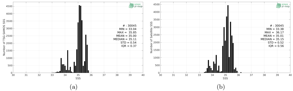
Figure 2: Histograms of SSS from TSG-SAMOS (a) and SMOS-L3-CATDS-CPDC-V3-MONTHLY-25KM (b) considering all match-up pairs per bins of 0.1 over the Roaring Forties and Furious Fifties Pi-MEP region and for the full satellite product period.
