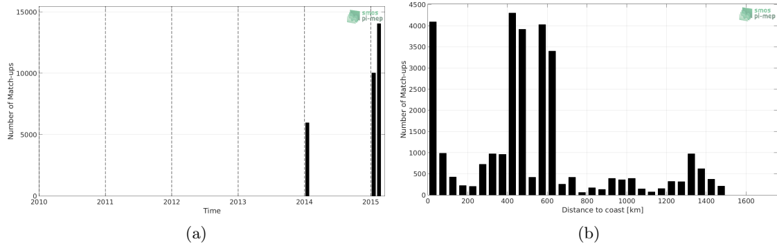
Figure 1: Number of match-ups between TSG-SAMOS and SMOS-L3-CATDS-CPDC-V3-MONTHLY-25KM SSS as a function of time (a) and as function of the distance to coast (b) over the Roaring Forties and Furious Fifties Pi-MEP region and for the full satellite product period.
