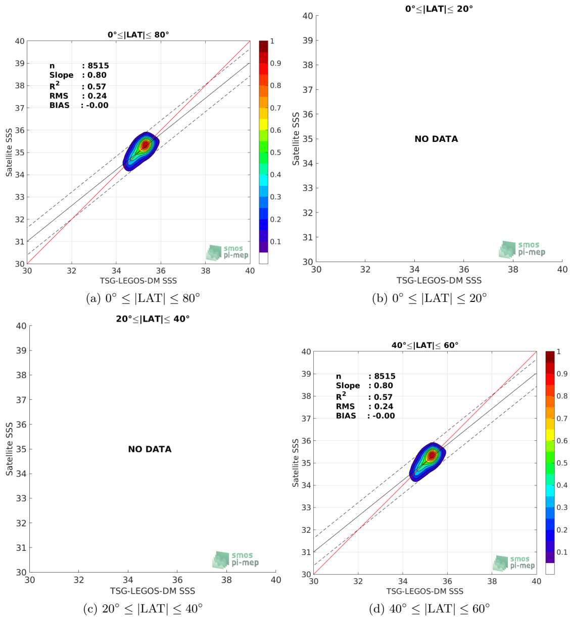
Figure 9: Contour maps of the concentration of SMOS-L3-CATDS-CPDC-V3-MONTHLY-25KM SSS (y-axis) versus TSG-LEGOS-DM SSS (x-axis) at match-up pairs for different latitude bands. For each plot, the red line shows x=y . The black thin and dashed lines indicate a linear fit through the data cloud and the \pm 95\% confidence levels, respectively. The number match-up pairs n , the slope and R^2 coefficient of the linear fit, the root mean square (RMS) and the mean bias between satellite and in situ data are indicated for each latitude band in each plots.
