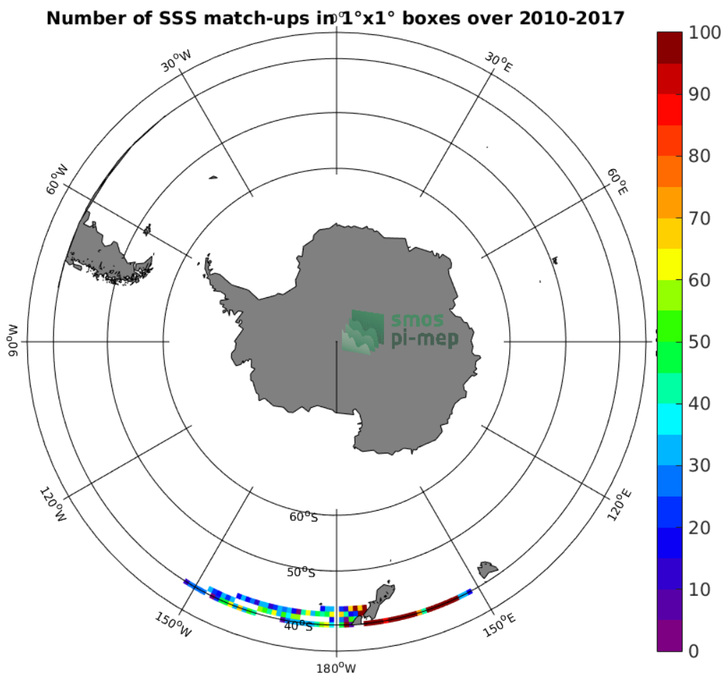
Figure 4: Number of SSS match-ups between TSG-LEGOS-DM SSS and the SMOS-L3-CATDS-CPDC-V3-MONTHLY-25KM SSS product for the Roaring Forties and Furious Fifties Pi-MEP region over 1^\circ \times 1^\circ boxes and for the full satellite product period.
