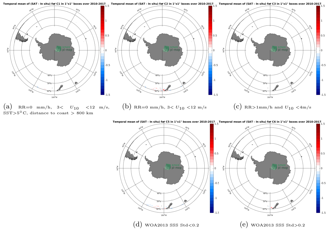
Figure 12: Temporal mean gridded over spatial boxes of size 1^\circ \times 1^\circ of \Delta SSS (SMOS-L3-CATDS-CPDC-V3-MONTHLY-25KM - TSG-LEGOS-DM) for 5 different subdatasets corresponding to:RR=0 mm/h, 3 < U_{10} < 12 m/s, SST >5^\circ C, distance to coast > 800 km (a), RR=0 mm/h, 3 < U_{10} < 12 m/s (b), RR >1 mm/h and U_{10} < 4 m/s (c), WOA2013 SSS Std <0.2 (d), WOA2013 SSS Std >0.2 (e).
