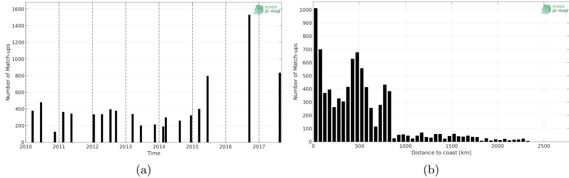
Figure 1: Number of match-ups between TSG-LEGOS-DM and SMOS-L3-CATDS-CPDC-V3-MONTHLY-25KM SSS as a function of time (a) and as function of the distance to coast (b) over the Roaring Forties and Furious Fifties Pi-MEP region and for the full satellite product period.
