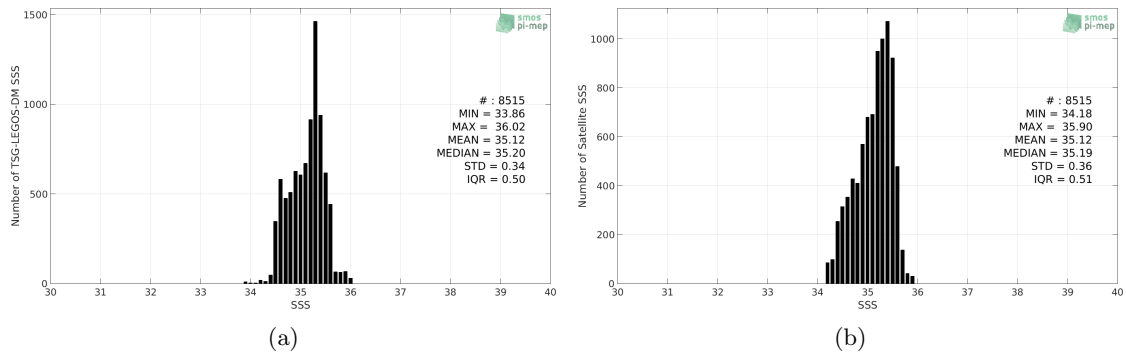
Figure 2: Histograms of SSS from TSG-LEGOS-DM (a) and SMOS-L3-CATDS-CPDC-V3-MONTHLY-25KM (b) considering all match-up pairs per bins of 0.1 over the Roaring Forties and Furious Fifties Pi-MEP region and for the full satellite product period.
