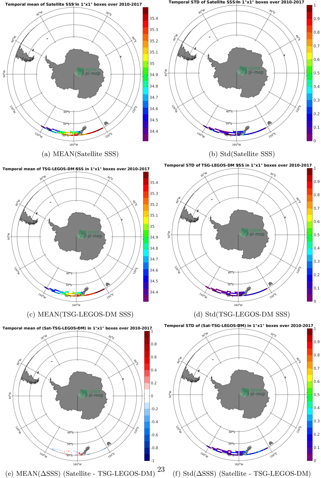
Figure 6: Temporal mean (left) and Std (right) of SSS from SMOS-L3-CATDS-CPDC-V3-MONTHLY-25KM (top), TSG-LEGOS-DM (middle), and of \Delta SSS (Satellite - TSG-LEGOS-DM). Only match-up pairs are used to generate these maps.
