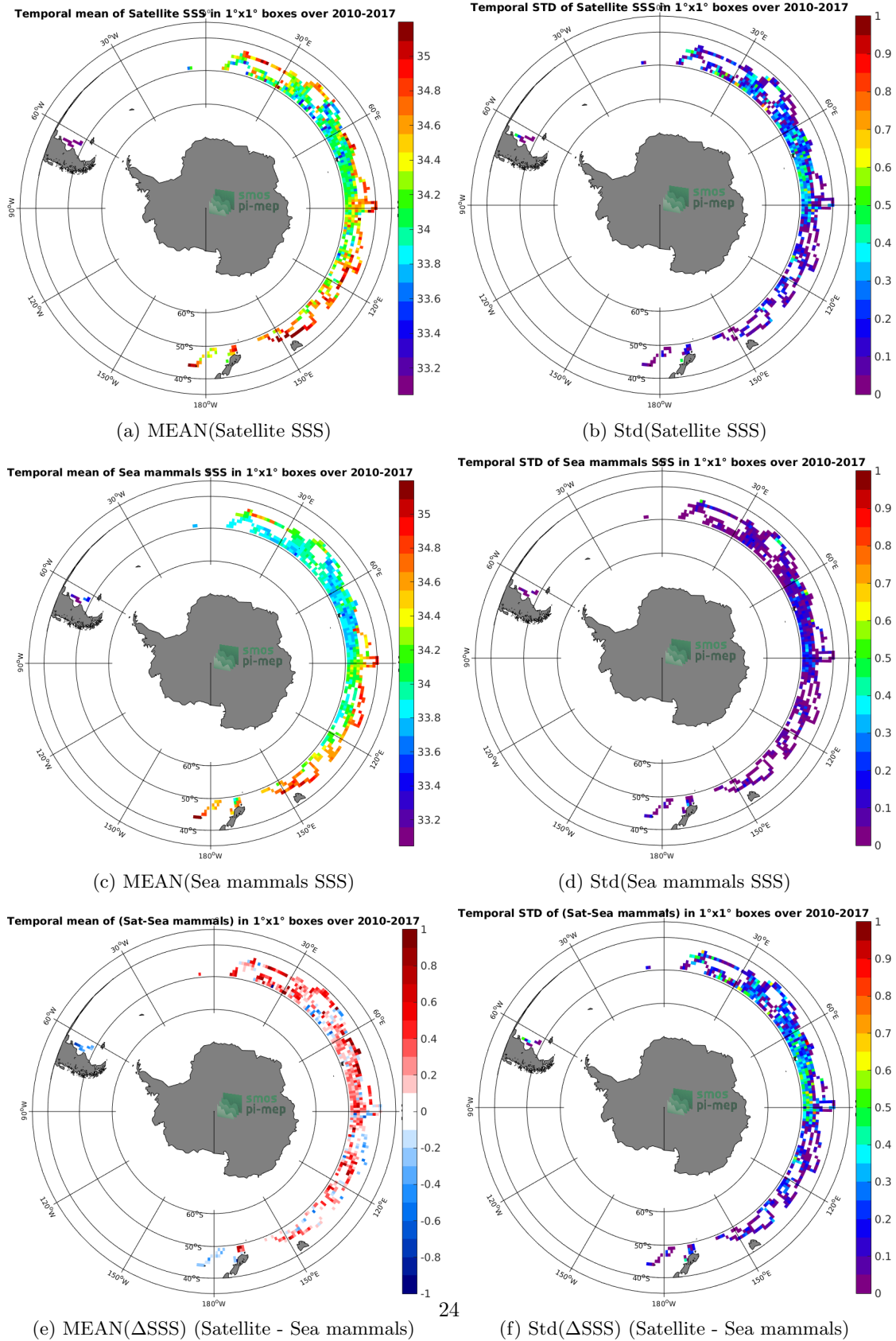
Figure 6: Temporal mean (left) and Std (right) of SSS from SMOS-L3-CATDS-CPDC-V3-MONTHLY-25KM (top), Sea mammals (middle), and of \Delta SSS (Satellite - Sea mammals). Only match-up pairs are used to generate these maps.
