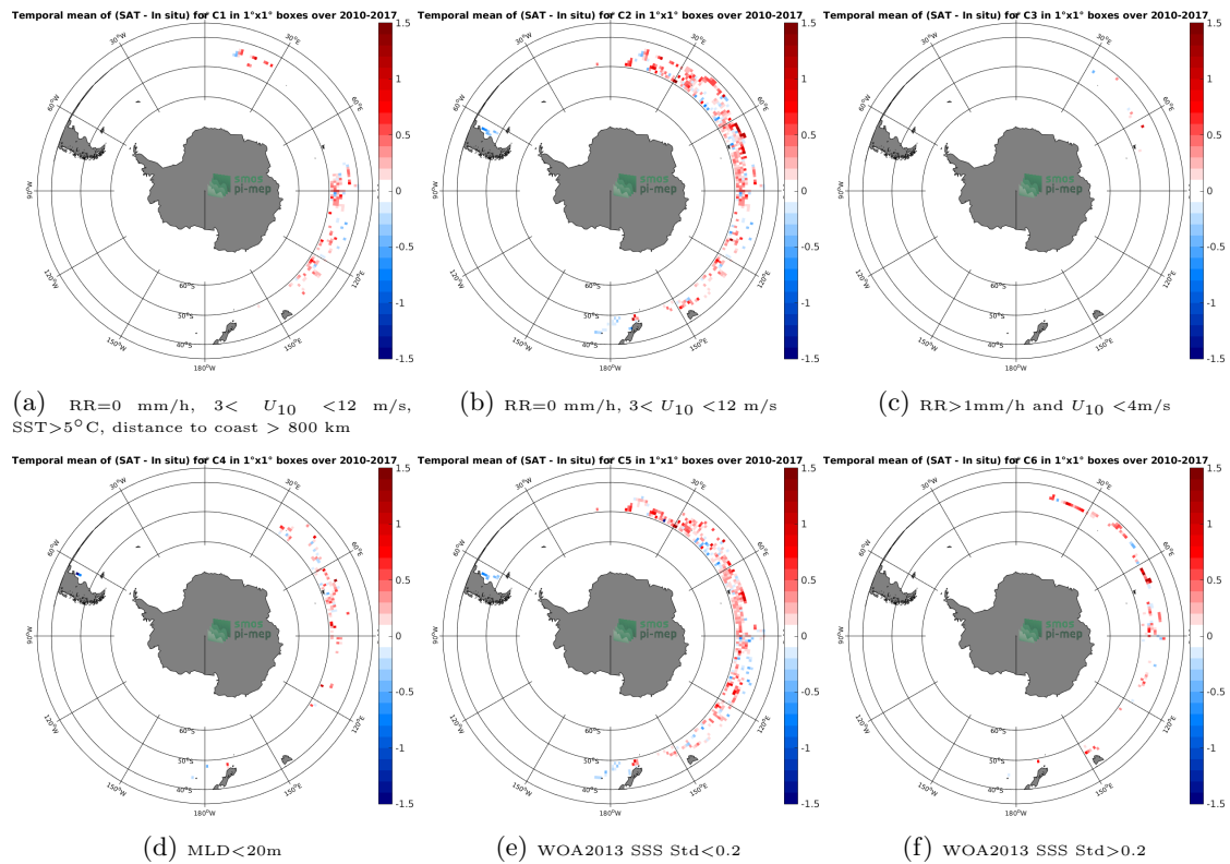
Figure 12: Temporal mean gridded over spatial boxes of size 1^\circ \times 1^\circ of \Delta SSS (SMOS-L3-CATDS-CPDC-V3-MONTHLY-25KM - Sea mammals) for 6 different subdatasets corresponding to:RR=0 mm/h, 3 < U_{10} < 12 m/s, SST >5^\circ C, distance to coast > 800 km (a), RR=0 mm/h, 3 < U_{10} < 12 m/s (b), RR >1 mm/h and U_{10} < 4 m/s (c),MLD <20 m (d),WOA2013 SSS Std <0.2 (e),WOA2013 SSS Std >0.2 (f).
