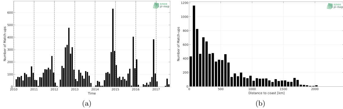
Figure 1: Number of match-ups between Sea mammals and SMOS-L3-CATDS-CPDC-V3-MONTHLY-25KM SSS as a function of time (a) and as function of the distance to coast (b) over the Roaring Forties and Furious Fifties Pi-MEP region and for the full satellite product period.
