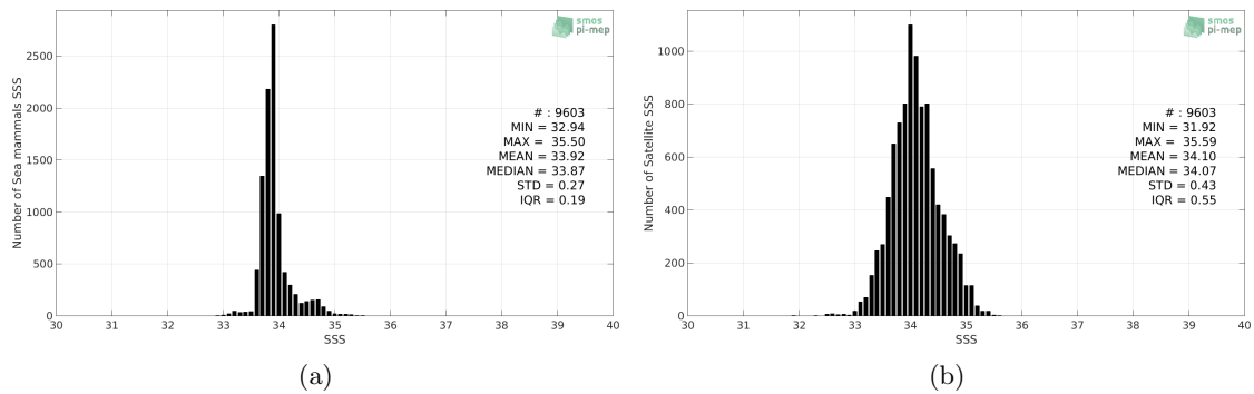
Figure 2: Histograms of SSS from Sea mammals (a) and SMOS-L3-CATDS-CPDC-V3-MONTHLY-25KM (b) considering all match-up pairs per bins of 0.1 over the Roaring Forties and Furious Fifties Pi-MEP region and for the full satellite product period.
