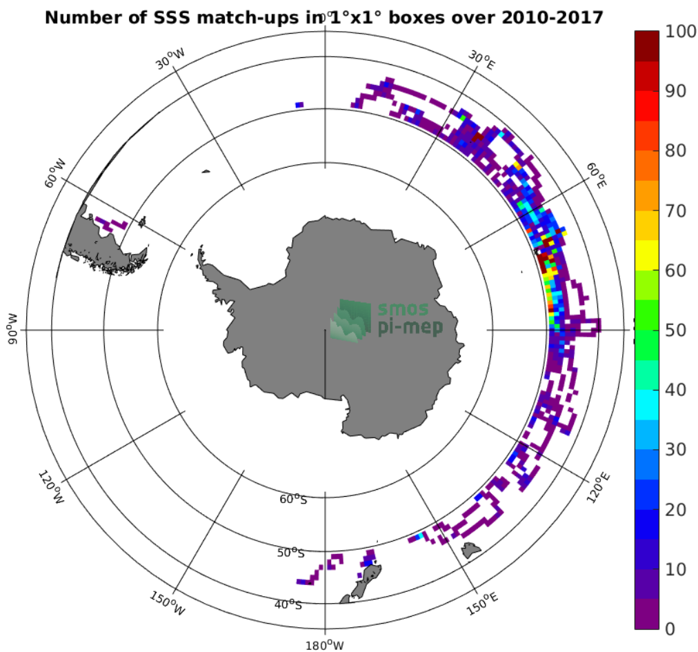
Figure 4: Number of SSS match-ups between Sea mammals SSS and the SMOS-L3-CATDS-CPDC-V3-MONTHLY-25KM SSS product for the Roaring Forties and Furious Fifties Pi-MEP region over 1°x1° boxes and for the full satellite product period.
