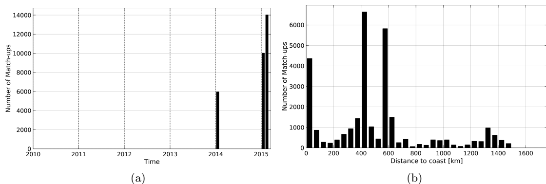
Figure 1: Number of match-ups between TSG-SAMOS and SMOS-L3-CATDS-CPDC-V3-10DAYS-25KM SSS as a function of time (a) and as function of the distance to the coast (b) over the Roaring Forties and Furious Fifties Pi-MEP region and for the full satellite product period.
