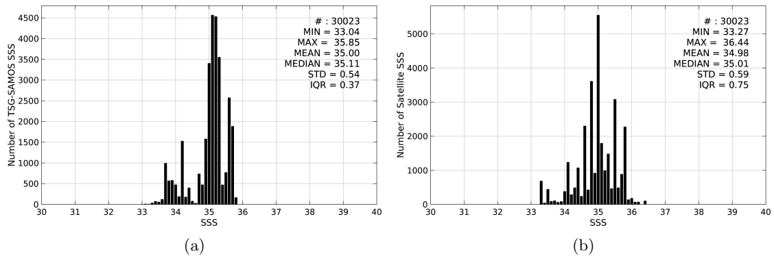
Figure 2: Histograms of SSS from TSG-SAMOS (a) and SMOS-L3-CATDS-CPDC-V3-10DAYS-25KM (b) considering all match-up pairs per bins of 0.1 over the Roaring Forties and Furious Fifties Pi-MEP region and for the full satellite product period.
