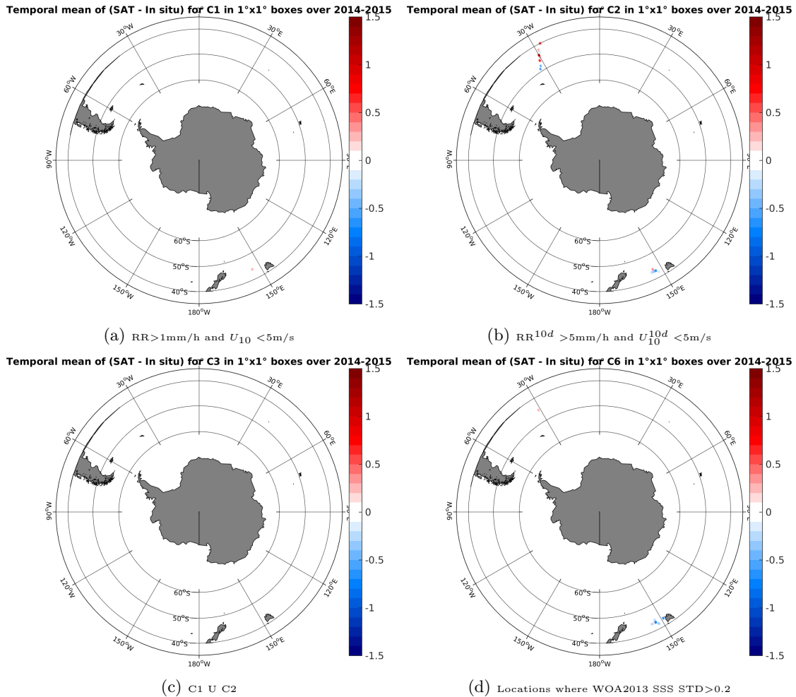
Figure 12: Temporal mean gridded over spatial boxes of size 1^\circ \times 1^\circ of \Delta SSS (SMOS-L3-CATDS-CPDC-V3-10DAYS-25KM - TSG-SAMOS) for 4 different subdatasets corresponding to: RR > 1\text{mm/h} and U_{10} < 5\text{m/s} (a), RR^{10d} > 5\text{mm/h} and U_{10}^{10d} < 5\text{m/s} (b), C1 U C2 (c), Locations where WOA2013 SSS STD > 0.2 (d).
