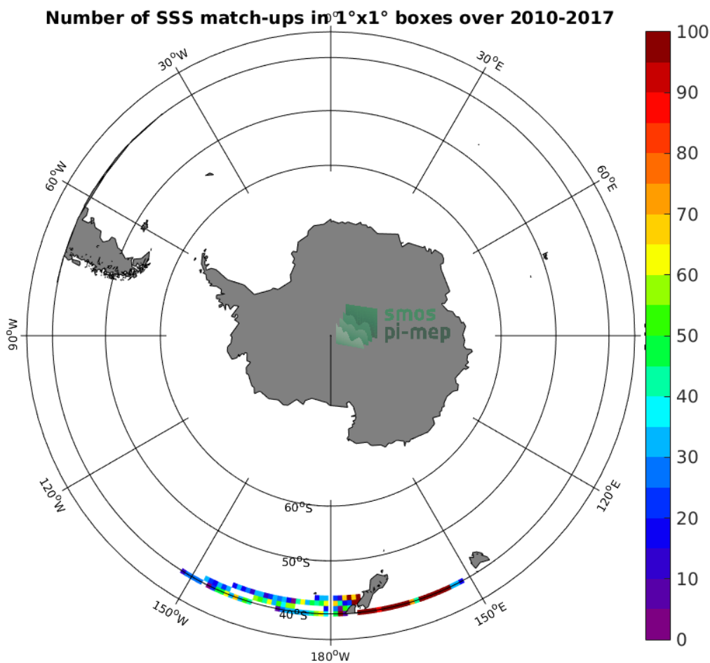
Figure 4: Number of SSS match-ups between TSG-LEGOS-DM SSS and the SMOS-L3-CATDS-CPDC-V3-10DAYS-25KM SSS product for the Roaring Forties and Furious Fifties Pi-MEP region over 1°x1° boxes and for the full satellite product period.
