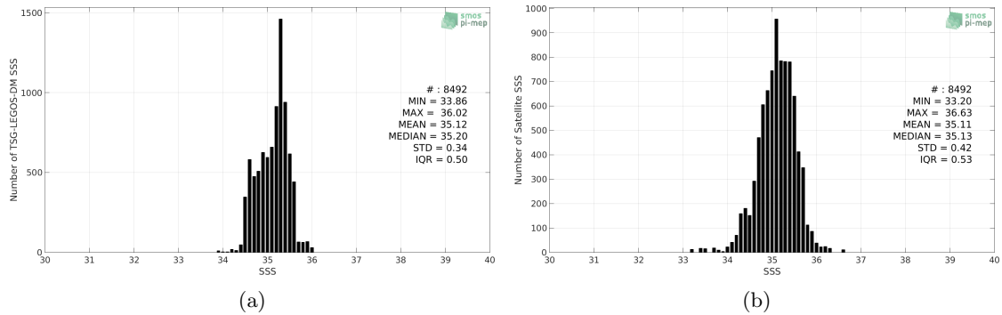
Figure 2: Histograms of SSS from TSG-LEGOS-DM (a) and SMOS-L3-CATDS-CPDC-V3-10DAYS-25KM (b) considering all match-up pairs per bins of 0.1 over the Roaring Forties and Furious Fifties Pi-MEP region and for the full satellite product period.
