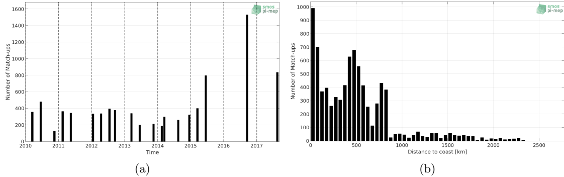
Figure 1: Number of match-ups between TSG-LEGOS-DM and SMOS-L3-CATDS-CPDC-V3-10DAYS-25KM SSS as a function of time (a) and as function of the distance to coast (b) over the Roaring Forties and Furious Fifties Pi-MEP region and for the full satellite product period.
