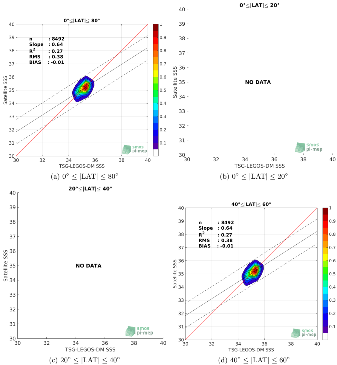
Figure 9: Contour maps of the concentration of SMOS-L3-CATDS-CPDC-V3-10DAYS-25KM SSS (y-axis) versus TSG-LEGOS-DM SSS (x-axis) at match-up pairs for different latitude bands. For each plot, the red line shows x=y . The black thin and dashed lines indicate a linear fit through the data cloud and the \pm 95\% confidence levels, respectively. The number match-up pairs n , the slope and R^2 coefficient of the linear fit, the root mean square (RMS) and the mean bias between satellite and in situ data are indicated for each latitude band in each plots.
