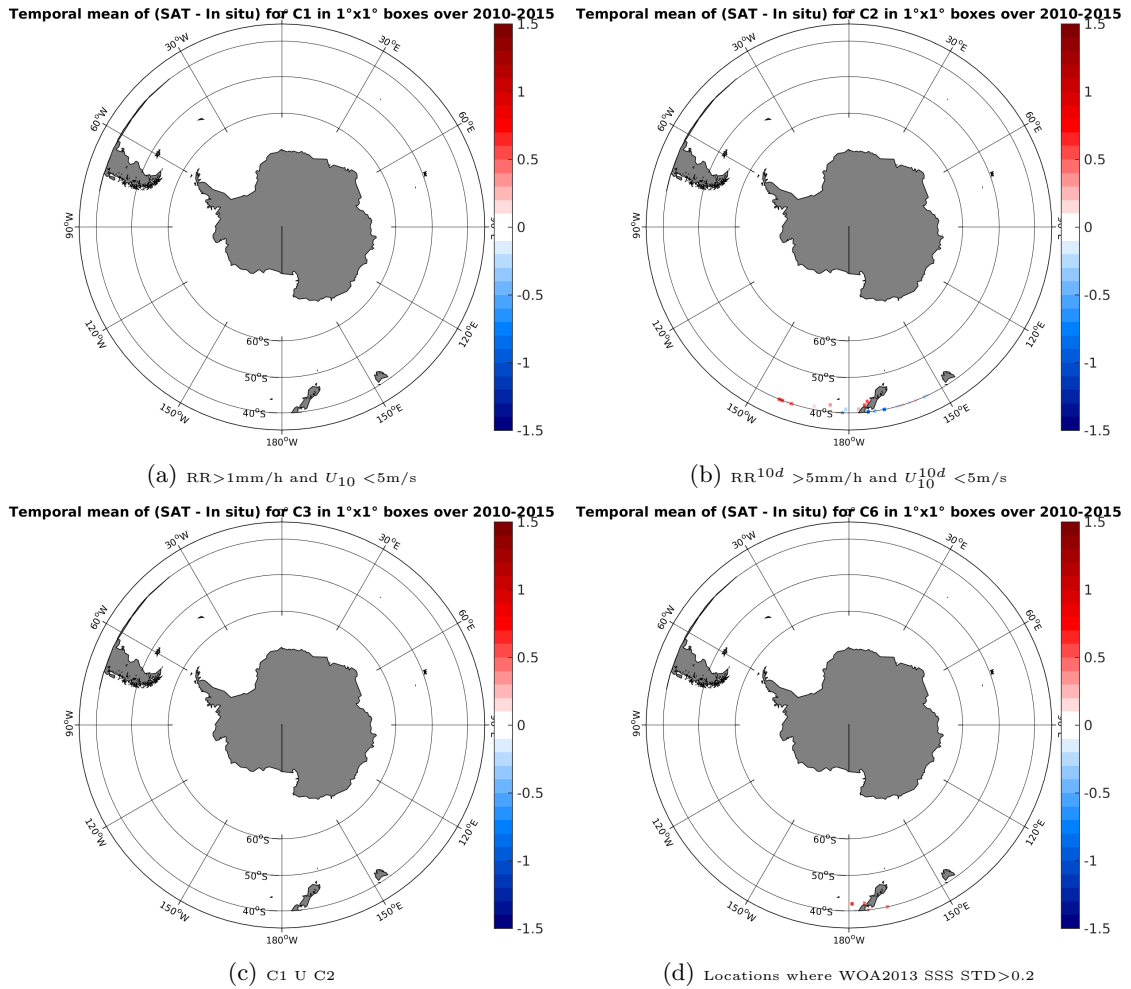
Figure 12: Temporal mean gridded over spatial boxes of size 1^\circ \times 1^\circ of \Delta SSS (SMOS-L3-CATDS-CPDC-V3-10DAYS-25KM - TSG-LEGOS-DM) for 4 different subdatasets corresponding to: RR > 1\text{mm/h} and U_{10} < 5\text{m/s} (a), RR^{10d} > 5\text{mm/h} and U_{10}^{10d} < 5\text{m/s} (b), C1 U C2 (c), Locations where WOA2013 SSS STD > 0.2 (d).
