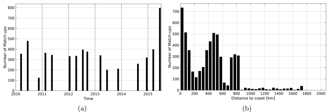
Figure 1: Number of match-ups between TSG-LEGOS-DM and SMOS-L3-CATDS-CPDC-V3-10DAYS-25KM SSS as a function of time (a) and as function of the distance to the coast (b) over the Roaring Forties and Furious Fifties Pi-MEP region and for the full satellite product period.
