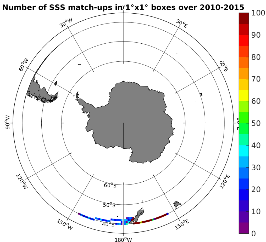
Figure 4: Number of SSS match-ups between TSG-LEGOS-DM SSS and the SMOS-L3-CATDS-CPDC-V3-10DAYS-25KM SSS product for the Roaring Forties and Furious Fifties Pi-MEP region over 1°x1° boxes and for the full satellite product period.
