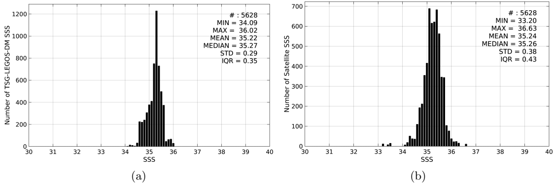
Figure 2: Histograms of SSS from TSG-LEGOS-DM (a) and SMOS-L3-CATDS-CPDC-V3-10DAYS-25KM (b) considering all match-up pairs per bins of 0.1 over the Roaring Forties and Furious Fifties Pi-MEP region and for the full satellite product period.
