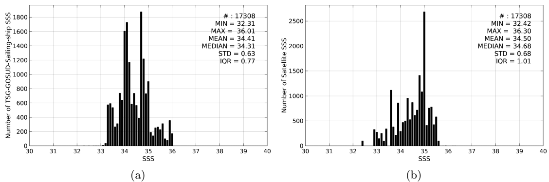
Figure 2: Histograms of SSS from TSG-GOSUD-Sailing-ship (a) and SMOS-L3-CATDS-CPDC-V3-10DAYS-25KM (b) considering all match-up pairs per bins of 0.1 over the Roaring Forties and Furious Fifties Pi-MEP region and for the full satellite product period.
