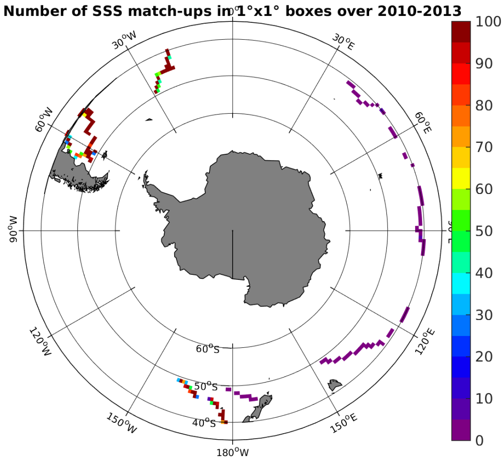
Figure 4: Number of SSS match-ups between TSG-GOSUD-Sailing-ship SSS and the SMOS-L3-CATDS-CPDC-V3-10DAYS-25KM SSS product for the Roaring Forties and Furious Fifties Pi-MEP region over 1^\circ \times 1^\circ boxes and for the full satellite product period.
