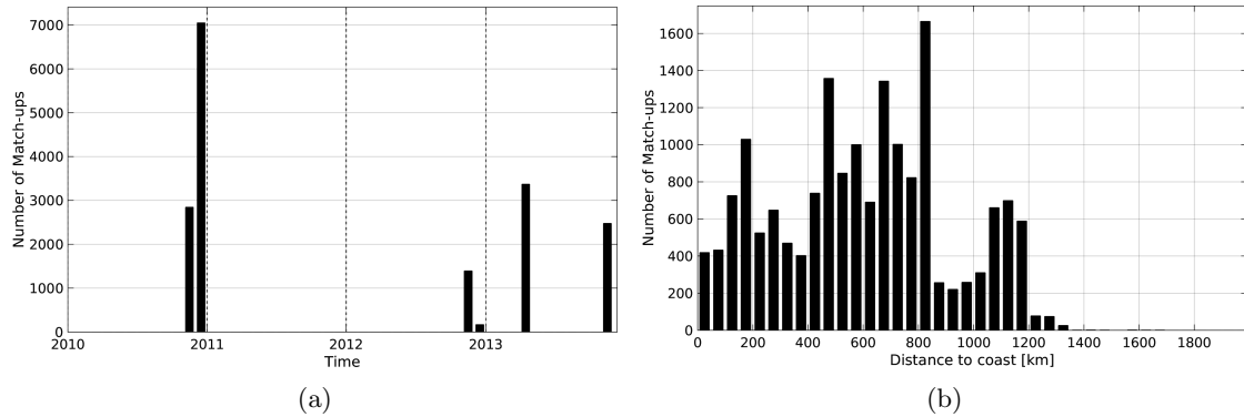
Figure 1: Number of match-ups between TSG-GOSUD-Sailing-ship and SMOS-L3-CATDS-CPDC-V3-10DAYS-25KM SSS as a function of time (a) and as function of the distance to coast (b) over the Roaring Forties and Furious Fifties Pi-MEP region and for the full satellite product period.
