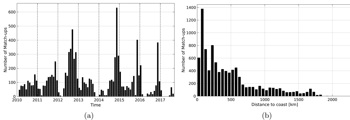
Figure 1: Number of match-ups between Sea mammals and SMOS-L3-CATDS-CPDC-V3-10DAYS-25KM SSS as a function of time (a) and as function of the distance to coast (b) over the Roaring Forties and Furious Fifties Pi-MEP region and for the full satellite product period.
