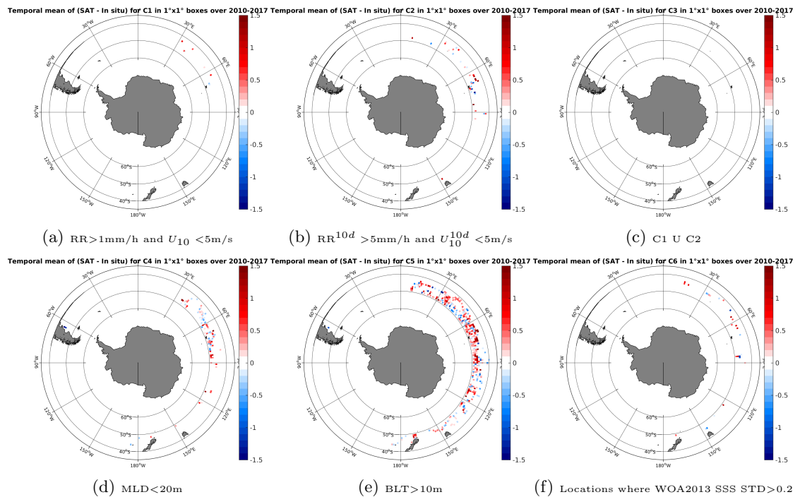
Figure 12: Temporal mean gridded over spatial boxes of size 1^\circ \times 1^\circ of \Delta SSS (SMOS-L3-CATDS-CPDC-V3-10DAYS-25KM - Sea mammals) for 6 different subdatasets corresponding to: RR > 1\text{mm/h} and U_{10} < 5\text{m/s} (a), RR^{10d} > 5\text{mm/h} and U_{10}^{10d} < 5\text{m/s} (b), C1 U C2 (c), MLD < 20\text{m} (d), BLT > 10\text{m} (e), Locations where WOA2013 SSS STD > 0.2 (f).
