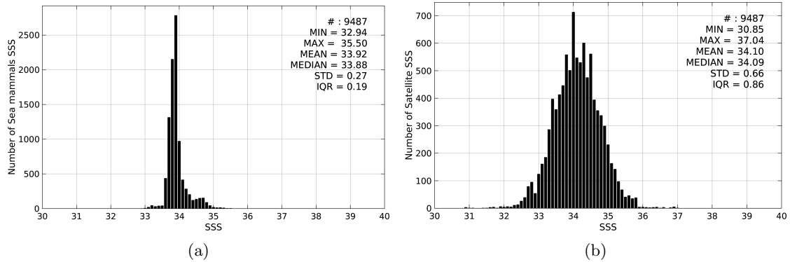
Figure 2: Histograms of SSS from Sea mammals (a) and SMOS-L3-CATDS-CPDC-V3-10DAYS-25KM (b) considering all match-up pairs per bins of 0.1 over the Roaring Forties and Furious Fifties Pi-MEP region and for the full satellite product period.
