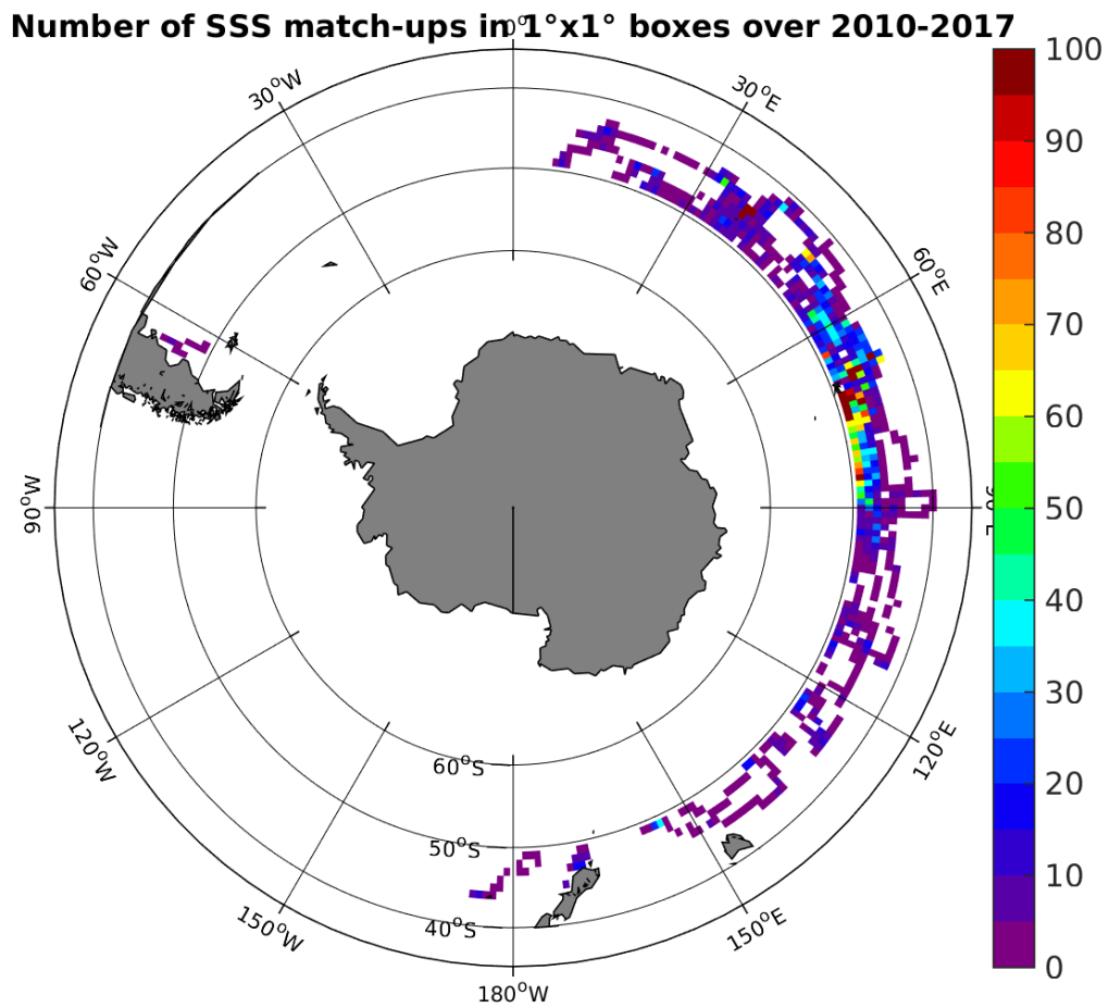
Figure 4: Number of SSS match-ups between Sea mammals SSS and the SMOS-L3-CATDS-CPDC-V3-10DAYS-25KM SSS product for the Roaring Forties and Furious Fifties Pi-MEP region over 1^\circ \times 1^\circ boxes and for the full satellite product period.
