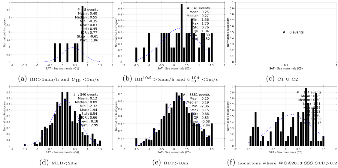
Figure 13: Normalized histogram of \Delta SSS (SMOS-L3-CATDS-CPDC-V3-10DAYS-25KM - Sea mammals) for 6 different subdatasets corresponding to: RR>1mm/h and U_{10} < 5\text{m/s} (a), RR^{10d} > 5\text{mm/h} and U_{10}^{10d} < 5\text{m/s} (b), C1 U C2 (c), MLD<20m (d), BLT>10m (e), Locations where WOA2013 SSS STD>0.2 (f).
