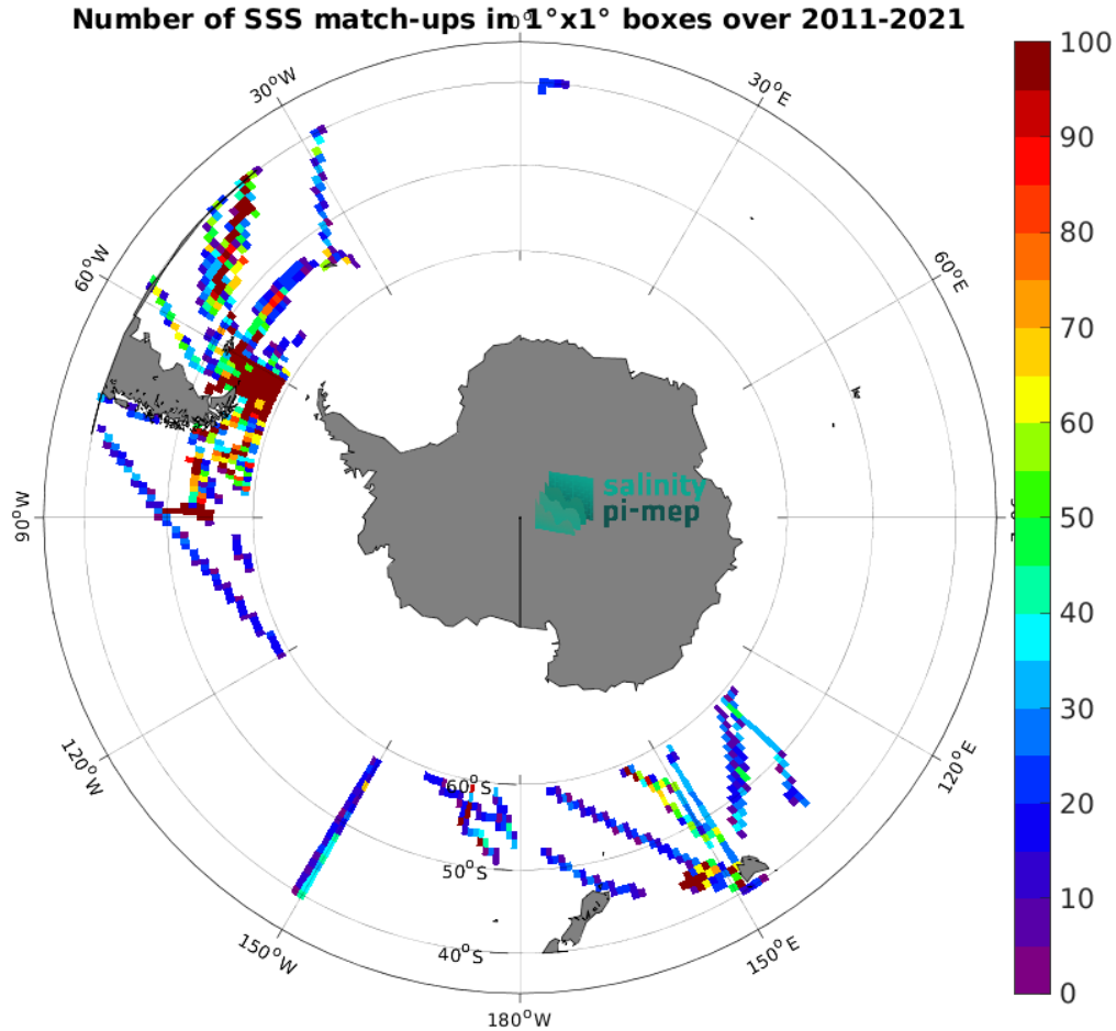
Figure 5: Number of SSS match-ups between TSG (SAMOS) SSS and the SMOS SSS L3 v2 - 9-Days (BEC) SSS product for the Roaring Forties and Furious Fifties Pi-MEP region over 1^\circ \times 1^\circ boxes and for the full satellite product period.
