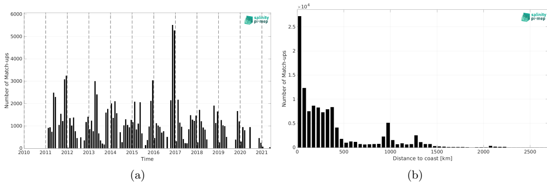
Figure 2: Number of match-ups between TSG (SAMOS) and SMOS SSS L3 v2 - 9-Days (BEC) SSS as a function of time (a) and as function of the distance to coast (b) over the Roaring Forties and Furious Fifties Pi-MEP region and for the full satellite product period.
