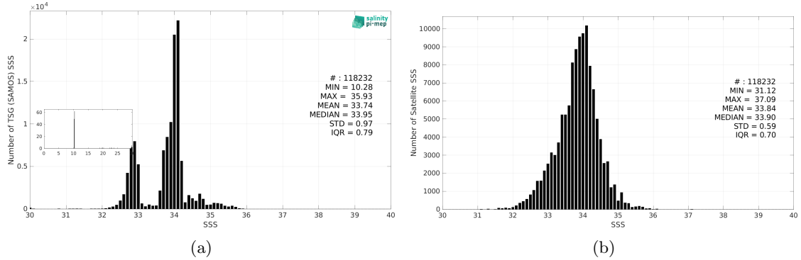
Figure 3: Histograms of SSS from TSG (SAMOS) (a) and SMOS SSS L3 v2 - 9-Days (BEC) (b) considering all match-up pairs per bins of 0.1 over the Roaring Forties and Furious Fifties Pi-MEP region and for the full satellite product period.
