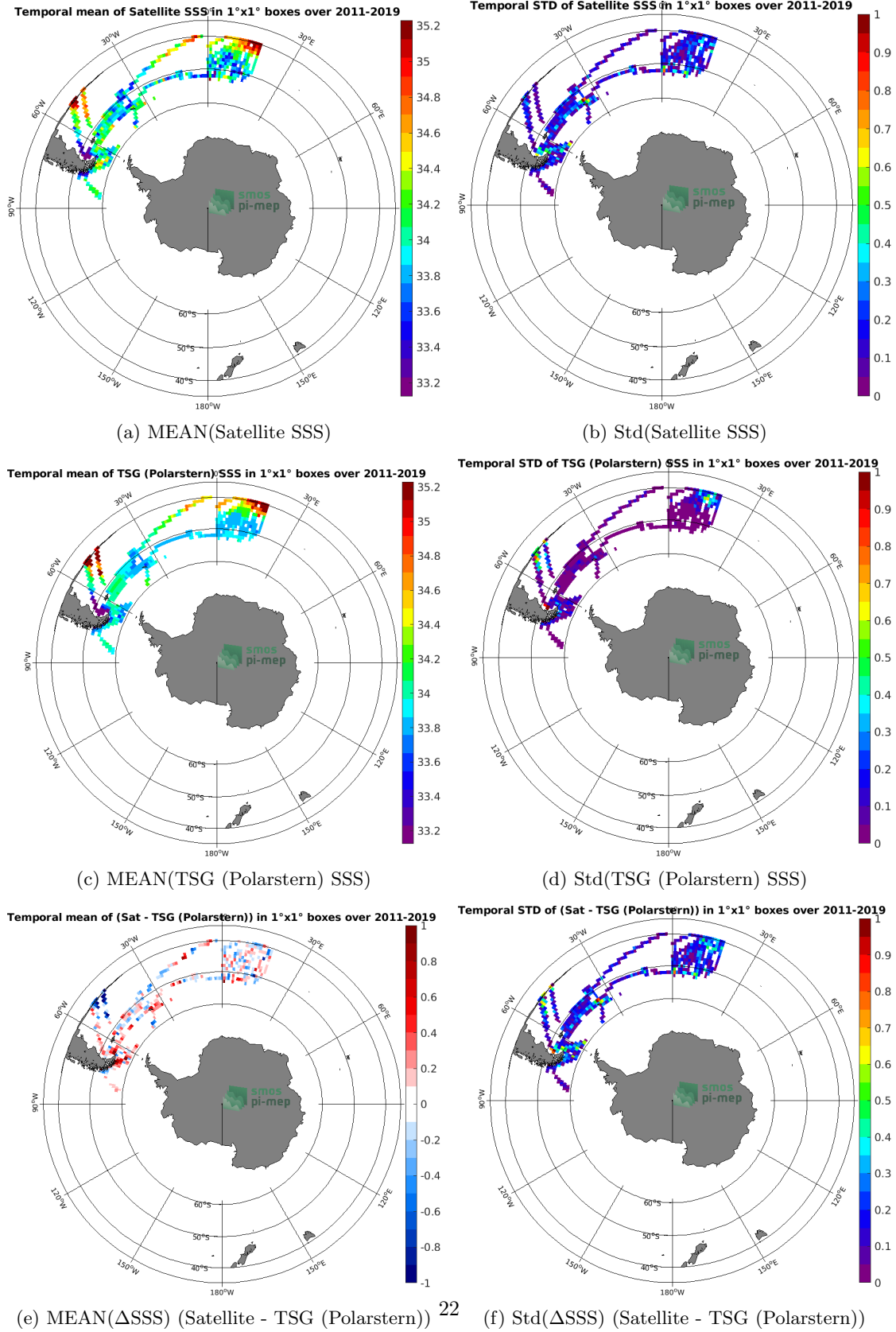
Figure 6: Temporal mean (left) and Std (right) of SSS from SMOS SSS L3 v2 - 9-Days (BEC) (top), TSG (Polarstern) (middle), and of \Delta SSS (Satellite - TSG (Polarstern)). Only match-up pairs are used to generate these maps.
