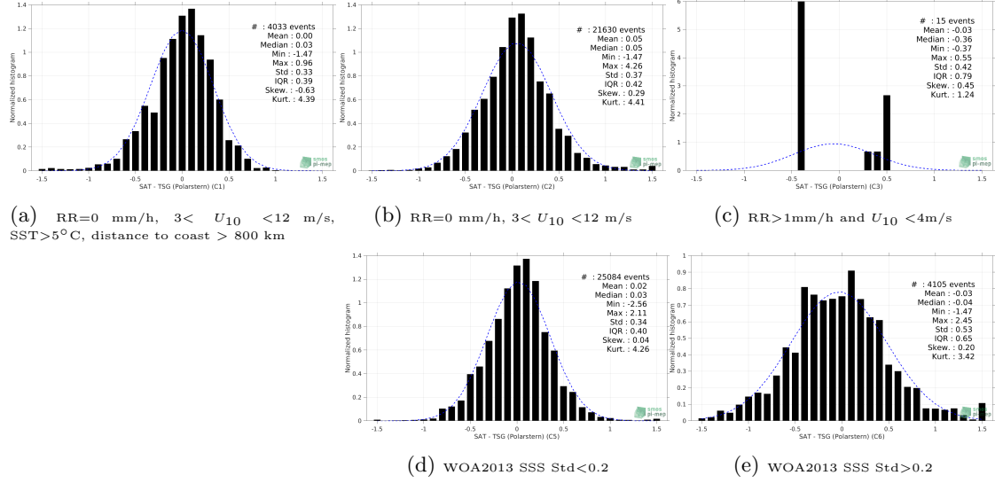
Figure 13: Normalized histogram of \Delta\text{SSS} (SMOS SSS L3 v2 - 9-Days (BEC) - TSG (Polarstern)) for 5 different subdatasets corresponding to: RR=0 mm/h, 3 < U_{10} < 12 m/s, SST>5°C, distance to coast > 800 km (a), RR=0 mm/h, 3 < U_{10} < 12 m/s (b), RR>1mm/h and U_{10} < 4 m/s (c), WOA2013 SSS Std<0.2 (d), WOA2013 SSS Std>0.2 (e).
