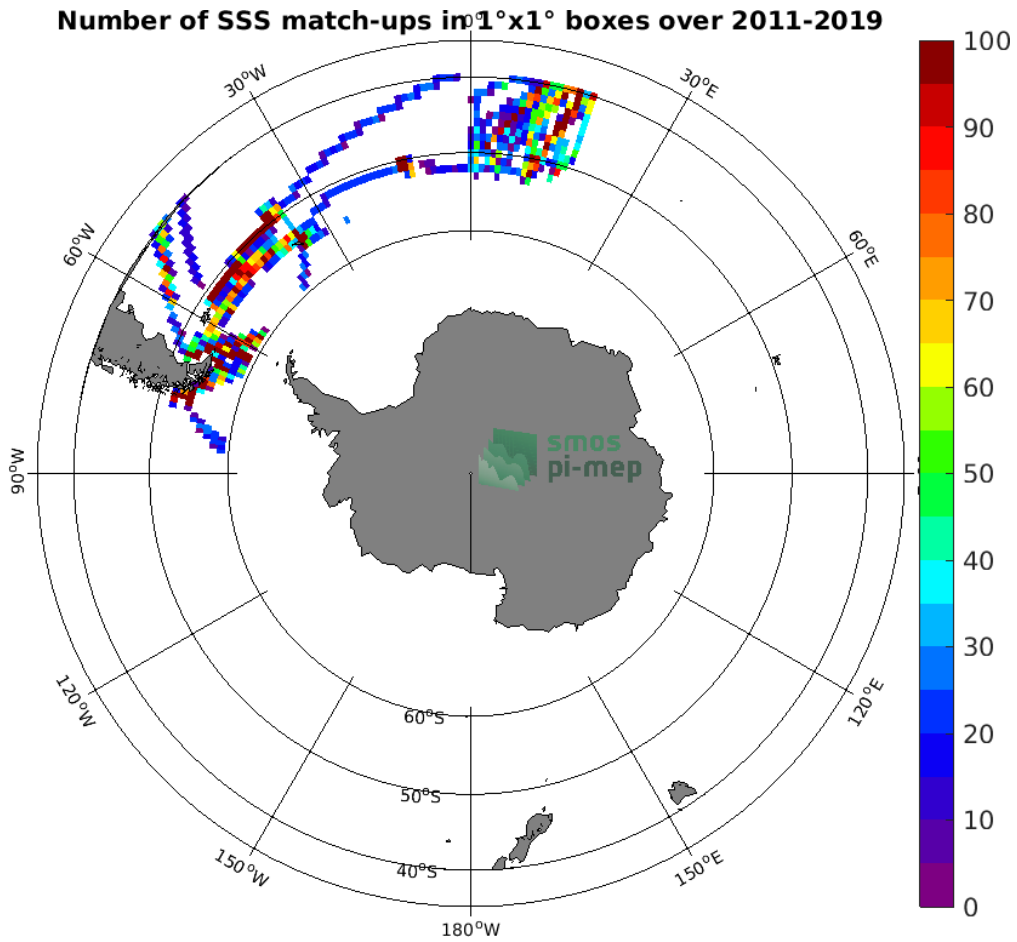
Figure 4: Number of SSS match-ups between TSG (Polarstern) SSS and the SMOS SSS L3 v2 - 9-Days (BEC) SSS product for the Roaring Forties and Furious Fifties Pi-MEP region over 1°x1° boxes and for the full satellite product period.
