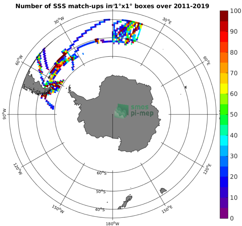
Figure 4: Number of SSS match-ups between TSG (Polarstern) SSS and the SMOS L3 v2 - 9-Days (BEC) SSS product for the Roaring Forties and Furious Fifties Pi-MEP region over 1^\circ \times 1^\circ boxes and for the full satellite product period.
