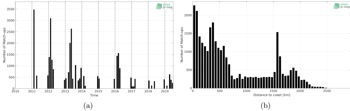
Figure 1: Number of match-ups between TSG (Polarstern) and SMOS L3 v2 - 9-Days (BEC) SSS as a function of time (a) and as function of the distance to coast (b) over the Roaring Forties and Furious Fifties Pi-MEP region and for the full satellite product period.
