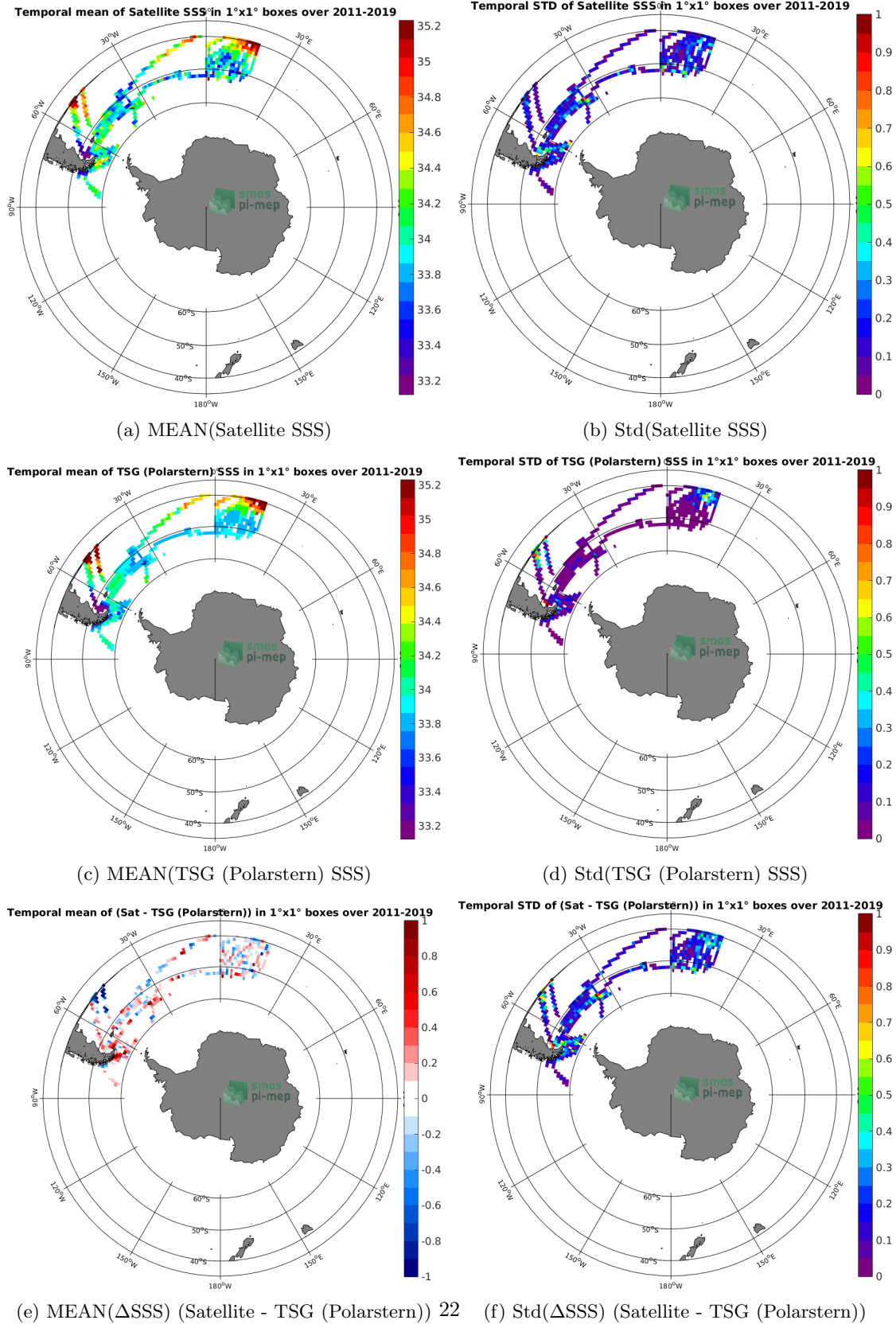
Figure 6: Temporal mean (left) and Std (right) of SSS from SMOS L3 v2 - 9-Days (BEC) (top), TSG (Polarstern) (middle), and of \Delta SSS (Satellite - TSG (Polarstern)). Only match-up pairs are used to generate these maps.
