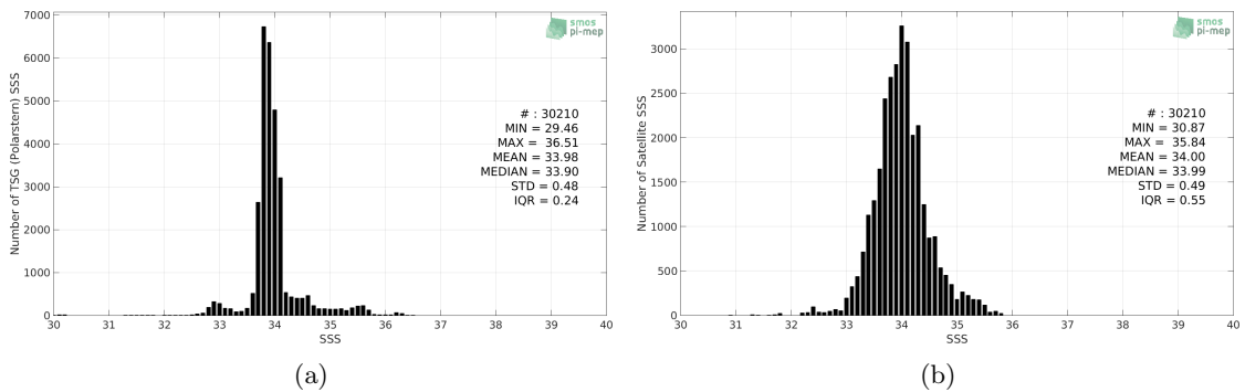
Figure 2: Histograms of SSS from TSG (Polarstern) (a) and SMOS L3 v2 - 9-Days (BEC) (b) considering all match-up pairs per bins of 0.1 over the Roaring Forties and Furious Fifties Pi-MEP region and for the full satellite product period.
