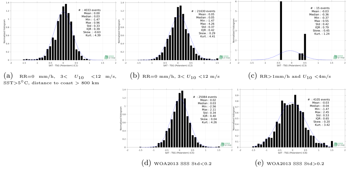
Figure 13: Normalized histogram of \Delta SSS (SMOS L3 v2 - 9-Days (BEC) - TSG (Polarstern)) for 5 different subdatasets corresponding to: RR=0 mm/h, 3 < U_{10} < 12 m/s, SST > 5°C, distance to coast > 800 km (a), RR=0 mm/h, 3 < U_{10} < 12 m/s (b), RR > 1mm/h and U_{10} < 4 m/s (c), WOA2013 SSS Std < 0.2 (d), WOA2013 SSS Std > 0.2 (e).
