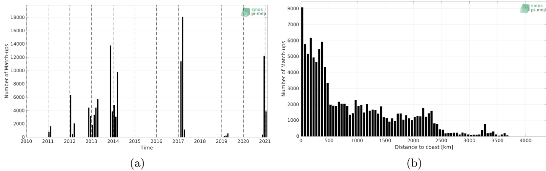
Figure 1: Number of match-ups between TSG (GOSUD-Sailing-ship) and SMOS SSS L3 v2 - 9-Days (BEC) SSS as a function of time (a) and as function of the distance to coast (b) over the Roaring Forties and Furious Fifties Pi-MEP region and for the full satellite product period.
