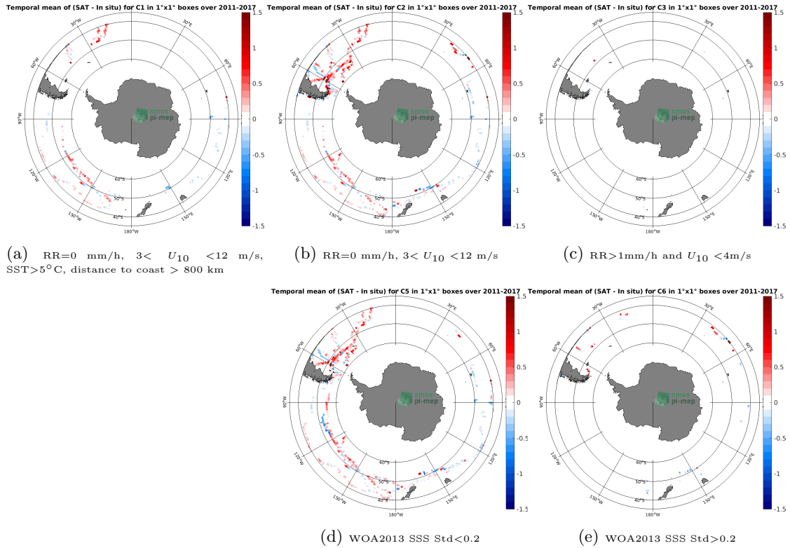
Figure 12: Temporal mean gridded over spatial boxes of size 1°x1° of \Delta SSS (SMOS SSS L3 v2 - 9-Days (BEC) - TSG (GOSUD-Sailing-ship)) for 5 different subdatasets corresponding to:RR=0 mm/h, 3 < U_{10} < 12 m/s, SST>5°C, distance to coast > 800 km (a), RR=0 mm/h, 3 < U_{10} < 12 m/s (b), RR>1mm/h and U_{10} < 4 m/s (c), WOA2013 SSS Std<0.2 (d), WOA2013 SSS Std>0.2 (e).
