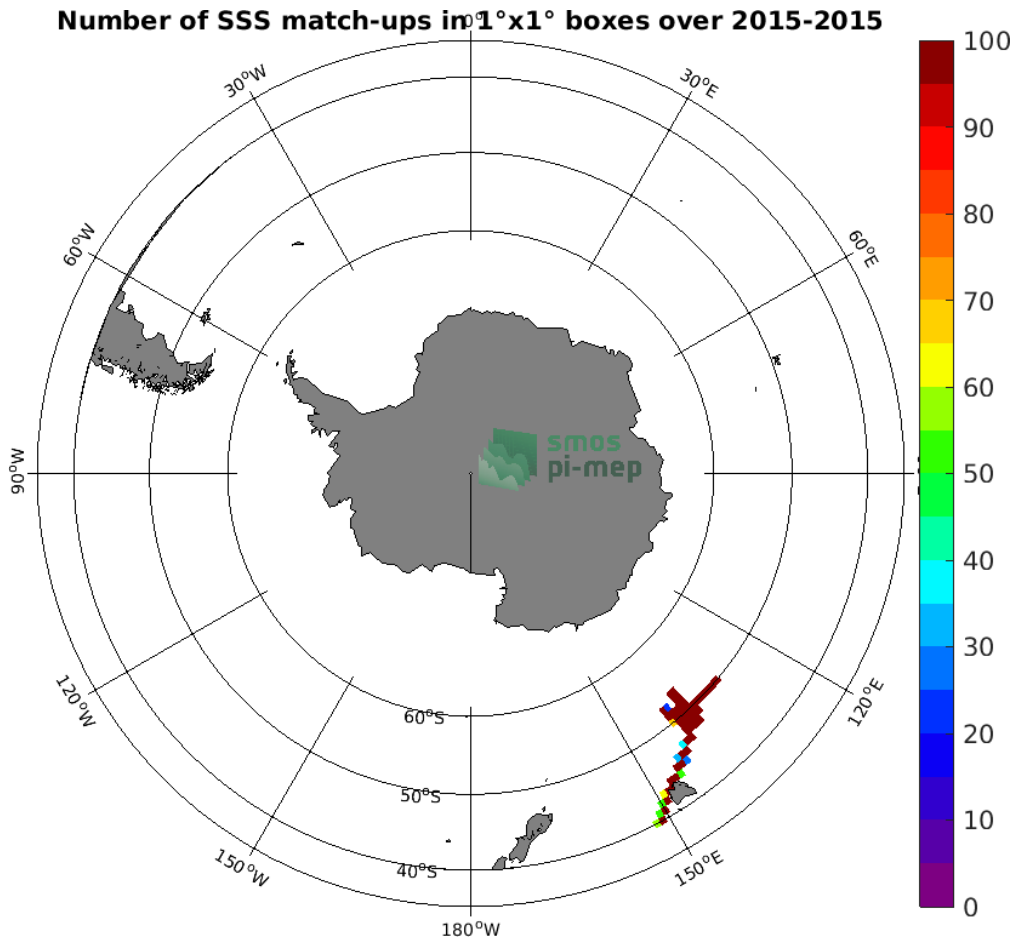
Figure 4: Number of SSS match-ups between TSG (GOSUD-Research-vessel) SSS and the SMOS SSS L3 v2 - 9-Days (BEC) SSS product for the Roaring Forties and Furious Fifties Pi-MEP region over 1°x1° boxes and for the full satellite product period.
