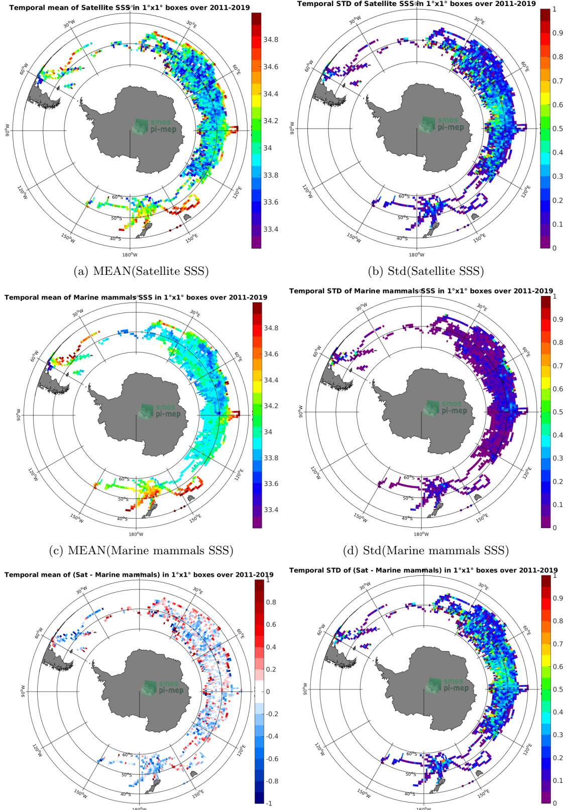
Figure 6: Temporal mean (left) and Std (right) of SSS from SMOS SSS L3 v2 - 9-Days (BEC) (top), Marine mammals (middle), and of \Delta SSS (Satellite - Marine mammals). Only match-up pairs are used to generate these maps.
