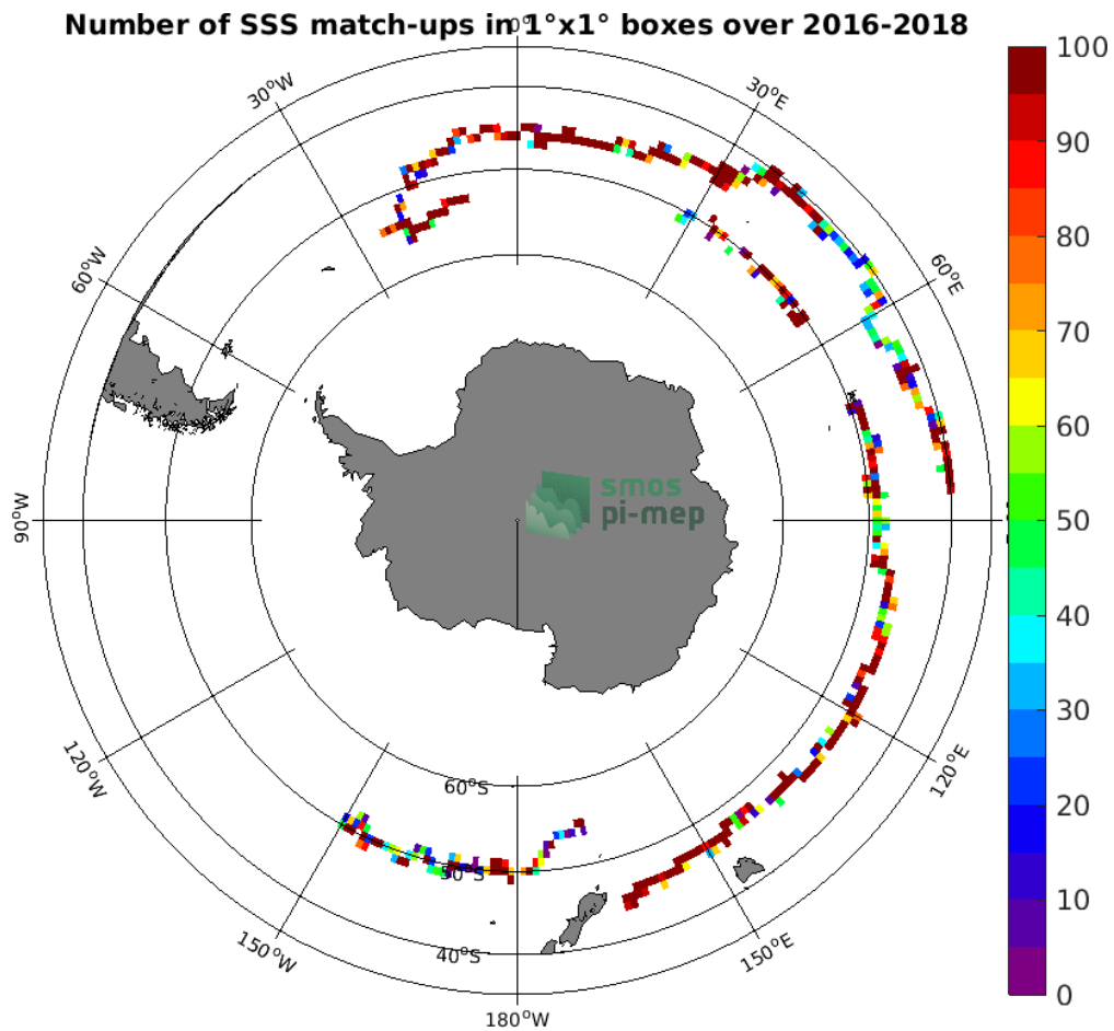
Figure 3: Number of SSS match-ups between Surface drifters SSS and the SMOS SSS L3 v2 - 9-Days (BEC) SSS product for the Roaring Forties and Furious Fifties Pi-MEP region over 1^\circ \times 1^\circ boxes and for the full satellite product period.
