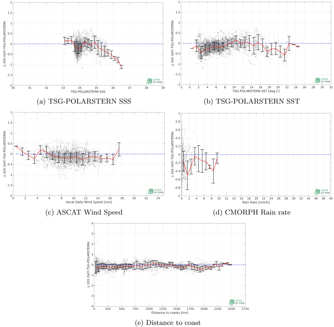
Figure 11: \Delta\text{SSS} (Satellite - TSG-POLARSTERN) sorted as function of TSG-POLARSTERN SSS values a), TSG-POLARSTERN SST b), ASCAT Wind speed c), CMORPH rain rate d) and distance to coast (e). In all plots the mean and Std of \Delta\text{SSS} for each bin is indicated by the red curves and black vertical thick bars ( \pm 1 Std)
