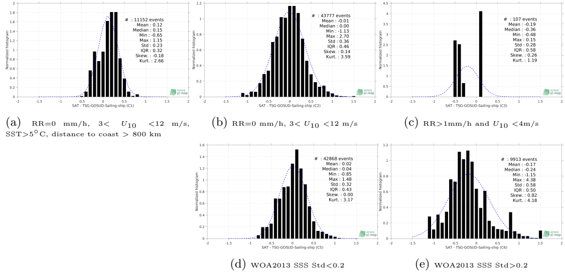
Figure 13: Normalized histogram of \Delta\text{SSS} (SMOS-L3-BEC-OA-V1-9DAYS-0.25DEG - TSG-GOSUD-Sailing-ship) for 5 different subdatasets corresponding to: RR=0 mm/h, 3 < U_{10} < 12 m/s, SST >5^{\circ}\text{C} , distance to coast > 800 km (a), RR=0 mm/h, 3 < U_{10} < 12 m/s (b), RR >1 mm/h and U_{10} < 4 m/s (c), WOA2013 SSS Std <0.2 (d), WOA2013 SSS Std >0.2 (e).
