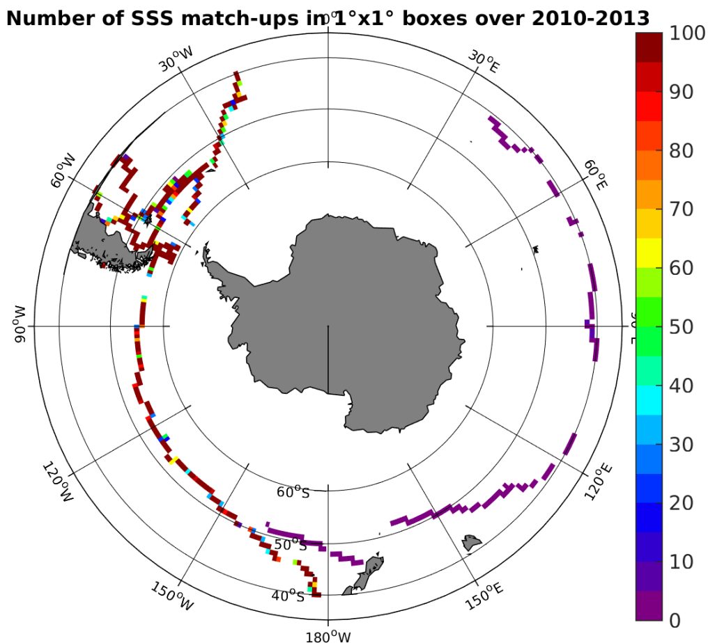
Figure 4: Number of SSS match-ups between TSG-GOSUD-Sailing-ship SSS and the SMOS-L3-BEC-OA-V1-9DAYS-0.25DEG SSS product for the Roaring Forties and Furious Fifties Pi-MEP region over 1^\circ \times 1^\circ boxes and for the full satellite product period.
