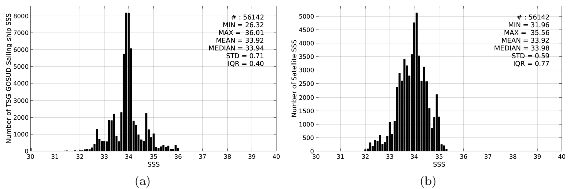
Figure 2: Histograms of SSS from TSG-GOSUD-Sailing-ship (a) and SMOS-L3-BEC-OA-V1-9DAYS-0.25DEG (b) considering all match-up pairs per bins of 0.1 over the Roaring Forties and Furious Fifties Pi-MEP region and for the full satellite product period.
