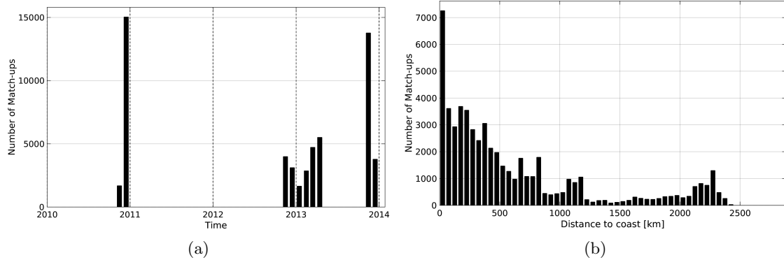
Figure 1: Number of match-ups between TSG-GOSUD-Sailing-ship and SMOS-L3-BEC-OA-V1-9DAYS-0.25DEG SSS as a function of time (a) and as function of the distance to coast (b) over the Roaring Forties and Furious Fifties Pi-MEP region and for the full satellite product period.
