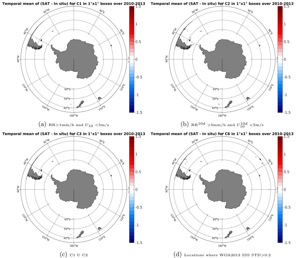
Figure 12: Temporal mean gridded over spatial boxes of size 1^\circ \times 1^\circ of \Delta SSS (SMOS-L3-BEC-OA-V1-9DAYS-0.25DEG - TSG-GOSUD-Sailing-ship) for 4 different subdatasets corresponding to: RR > 1\text{mm/h} and U_{10} < 5\text{m/s} (a), RR^{10d} > 5\text{mm/h} and U_{10}^{10d} < 5\text{m/s} (b), C1 U C2 (c), Locations where WOA2013 SSS STD > 0.2 (d).
