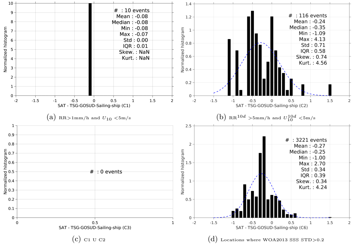
Figure 13: Normalized histogram of \Delta\text{SSS} (SMOS-L3-BEC-OA-V1-9DAYS-0.25DEG - TSG-GOSUD-Sailing-ship) for 6 different subdatasets corresponding to: RR > 1\text{mm/h} and U_{10} < 5\text{m/s} (a), RR^{10d} > 5\text{mm/h} and U_{10}^{10d} < 5\text{m/s} (b), C1 \cup C2 (c), Locations where WOA2013 SSS STD > 0.2 (d).
