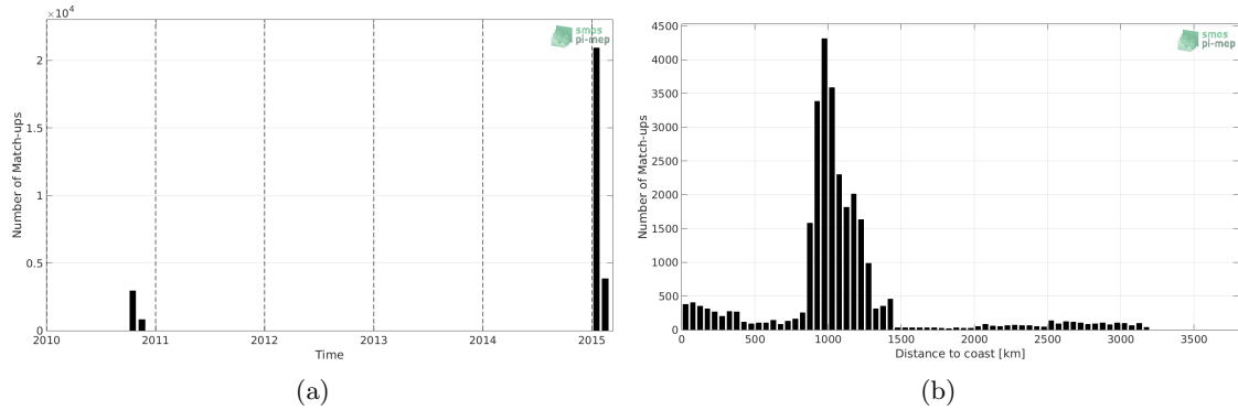
Figure 1: Number of match-ups between TSG-GOSUD-Research-vessel and SMOS-L3-BEC-OA-V1-9DAYS-0.25DEG SSS as a function of time (a) and as function of the distance to coast (b) over the Roaring Forties and Furious Fifties Pi-MEP region and for the full satellite product period.
