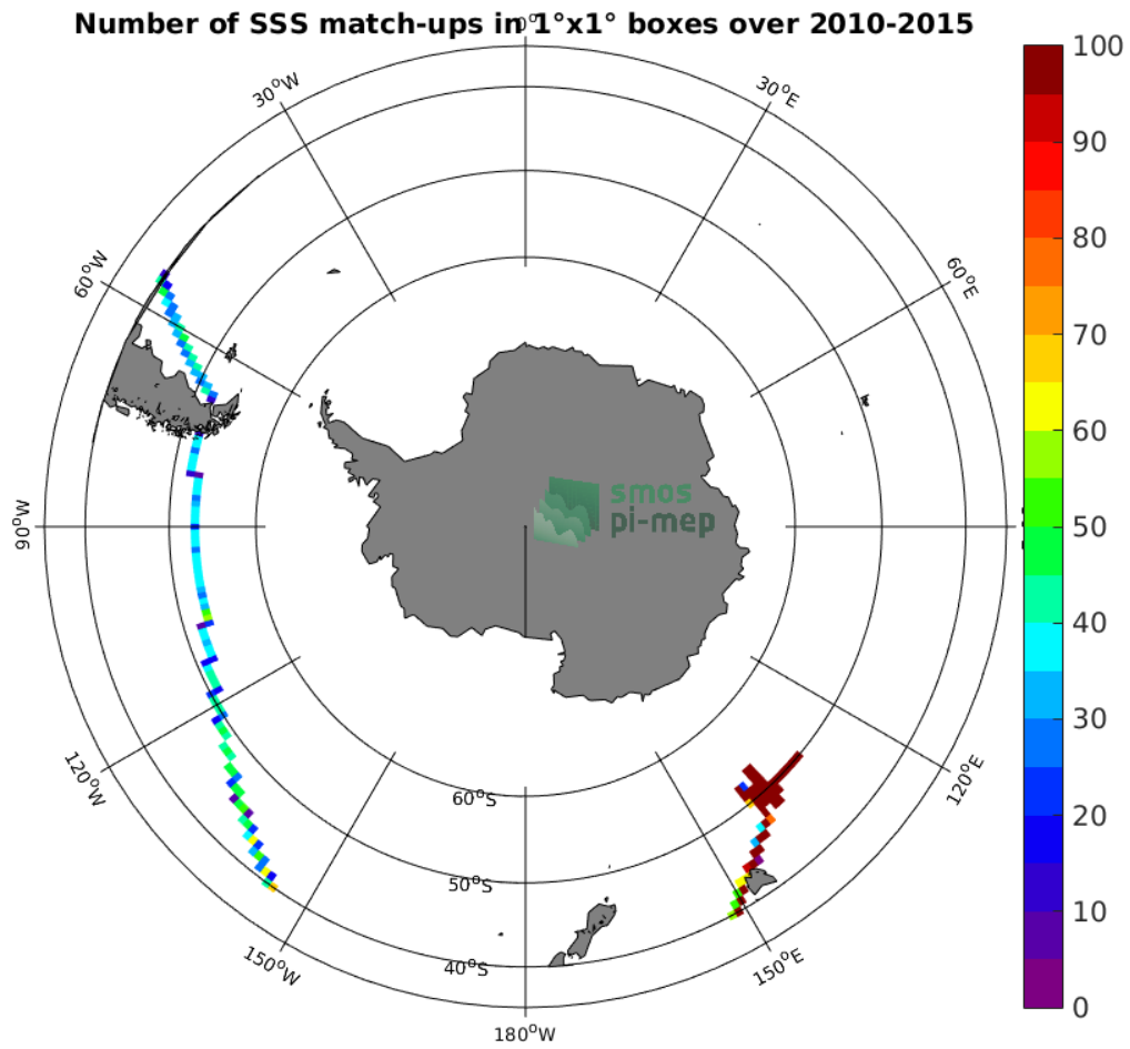
Figure 4: Number of SSS match-ups between TSG-GOSUD-Research-vessel SSS and the SMOS-L3-BEC-OA-V1-9DAYS-0.25DEG SSS product for the Roaring Forties and Furious Fifties Pi-MEP region over 1°x1° boxes and for the full satellite product period.
