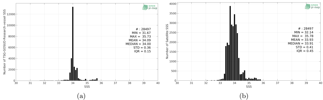
Figure 2: Histograms of SSS from TSG-GOSUD-Research-vessel (a) and SMOS-L3-BEC-OA-V1-9DAYS-0.25DEG (b) considering all match-up pairs per bins of 0.1 over the Roaring Forties and Furious Fifties Pi-MEP region and for the full satellite product period.
