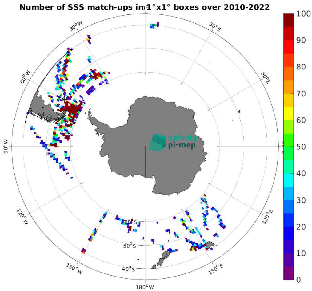
Figure 5: Number of SSS match-ups between TSG (SAMOS) SSS and the SMOS SSS L2 v700 (ESA) SSS product for the Roaring Forties and Furious Fifties Pi-MEP region over 1^\circ \times 1^\circ boxes and for the full satellite product period.
