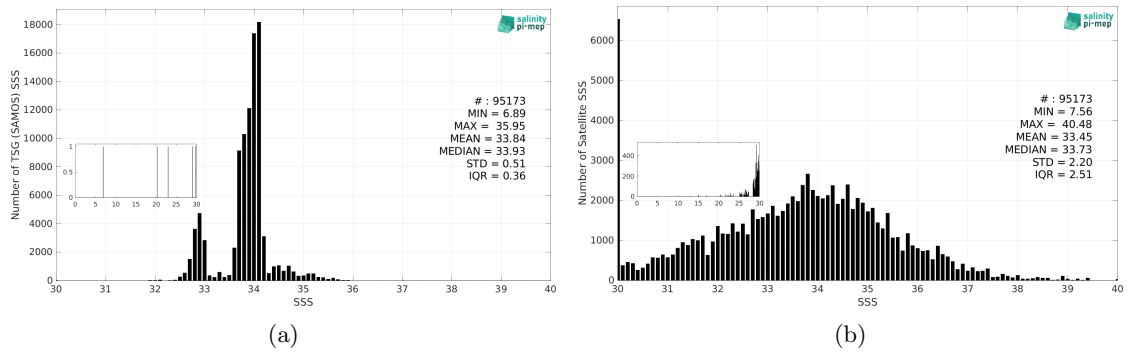
Figure 3: Histograms of SSS from TSG (SAMOS) (a) and SMOS SSS L2 v700 (ESA) (b) considering all match-up pairs per bins of 0.1 over the Roaring Forties and Furious Fifties Pi-MEP region and for the full satellite product period.
