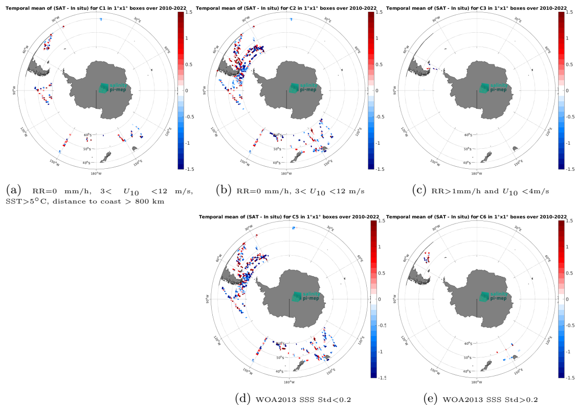
Figure 14: Temporal mean gridded over spatial boxes of size 1^\circ \times 1^\circ of \Delta SSS (SMOS SSS L2 v700 (ESA) - TSG (SAMOS)) for 5 different subdatasets corresponding to:RR=0 mm/h, 3 < U_{10} < 12 m/s, SST>5°C, distance to coast > 800 km (a), RR=0 mm/h, 3 < U_{10} < 12 m/s (b), RR>1mm/h and U_{10} < 4 m/s (c), WOA2013 SSS Std<0.2 (d), WOA2013 SSS Std>0.2 (e).
