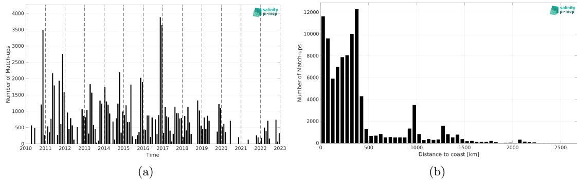
Figure 2: Number of match-ups between TSG (SAMOS) and SMOS SSS L2 v700 (ESA) SSS as a function of time (a) and as function of the distance to coast (b) over the Roaring Forties and Furious Fifties Pi-MEP region and for the full satellite product period.
