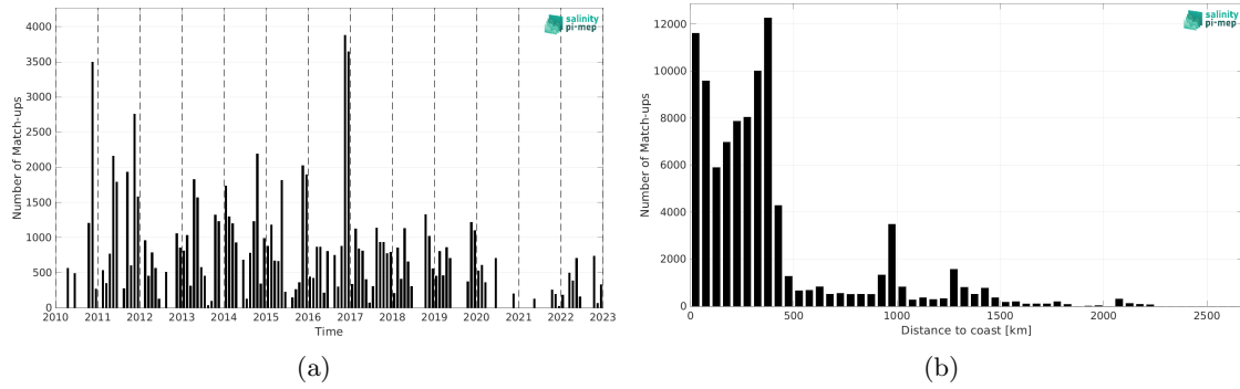
Figure 1: Number of match-ups between TSG (SAMOS) and SMOS SSS L2 v700 (ESA) SSS as a function of time (a) and as function of the distance to coast (b) over the Roaring Forties and Furious Fifties Pi-MEP region and for the full satellite product period.
