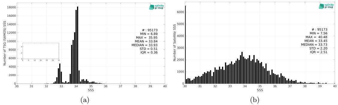
Figure 2: Histograms of SSS from TSG (SAMOS) (a) and SMOS SSS L2 v700 (ESA) (b) considering all match-up pairs per bins of 0.1 over the Roaring Forties and Furious Fifties Pi-MEP region and for the full satellite product period.
