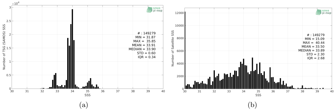
Figure 2: Histograms of SSS from TSG (SAMOS) (a) and SMOS SSS L2 v700 (ESA) (b) considering all match-up pairs per bins of 0.1 over the Roaring Forties and Furious Fifties Pi-MEP region and for the full satellite product period.
