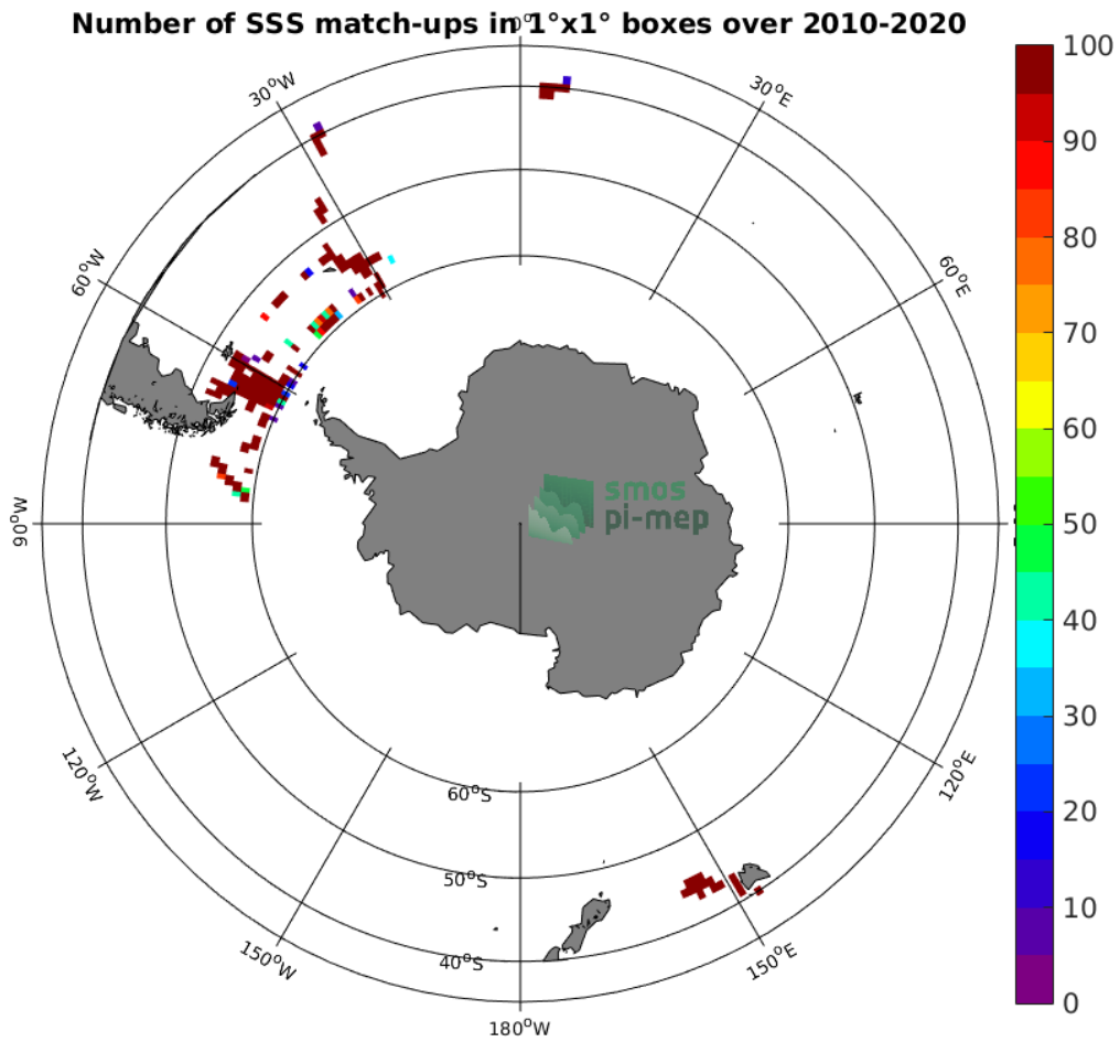
Figure 4: Number of SSS match-ups between TSG (SAMOS) SSS and the SMOS SSS L2 v700 (ESA) SSS product for the Roaring Forties and Furious Fifties Pi-MEP region over 1^\circ \times 1^\circ boxes and for the full satellite product period.
