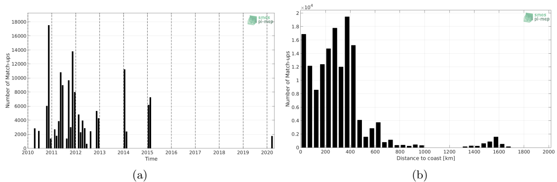
Figure 1: Number of match-ups between TSG (SAMOS) and SMOS SSS L2 v700 (ESA) SSS as a function of time (a) and as function of the distance to coast (b) over the Roaring Forties and Furious Fifties Pi-MEP region and for the full satellite product period.
