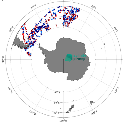
(e) MEAN( \Delta SSS) (Satellite - TSG (Polarstern)) 20
